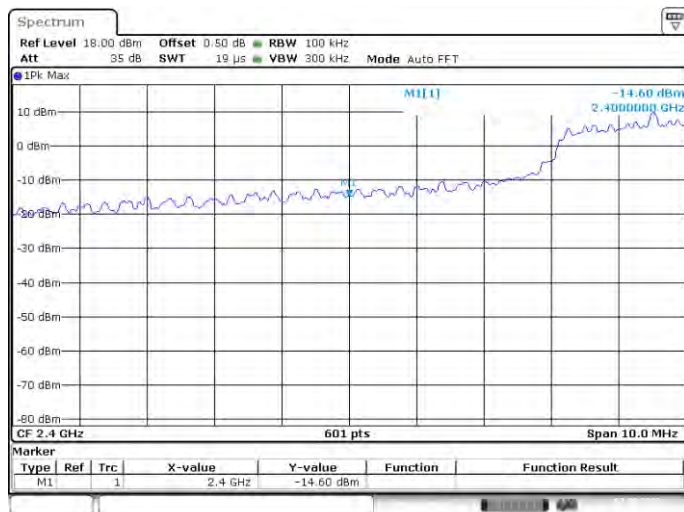
802.11n-20 LOW CHANNEL, Band Edge
