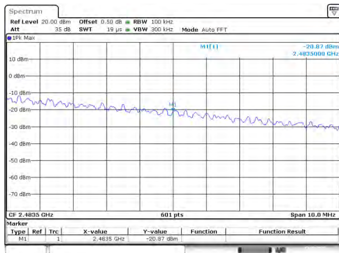
802.11n-20 HIGH CHANNEL, Band Edge
