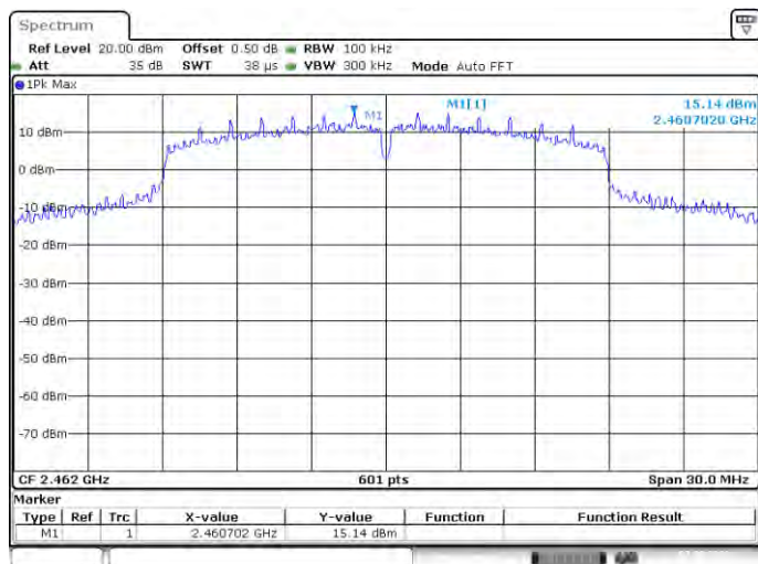
802.11n-20 HIGH CHANNEL, Carrier level
