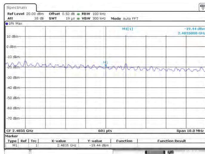
802.11n-40 MHz HIGH CHANNEL, Band Edge
