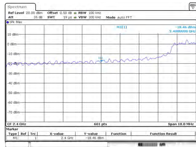
802.11n-40 MHz LOW CHANNEL, Band Edge
