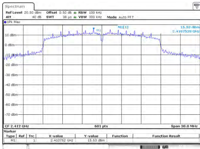
802.11n-20 LOW CHANNEL, Carrier level
