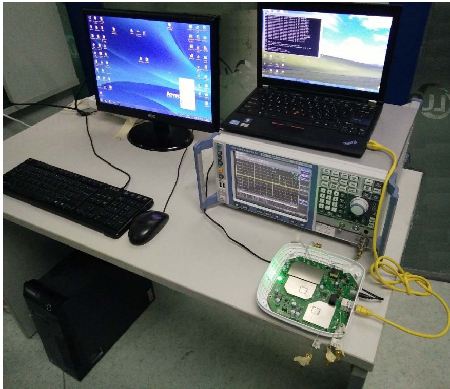
Conducted Test
