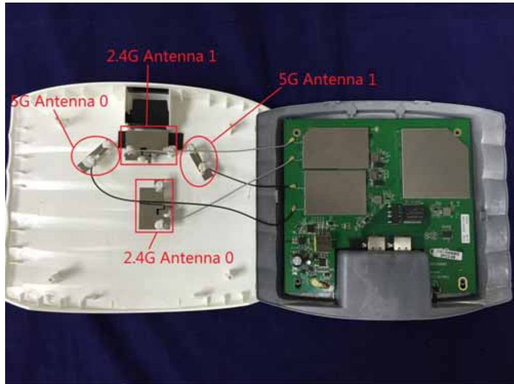
(1) EUT Photo
