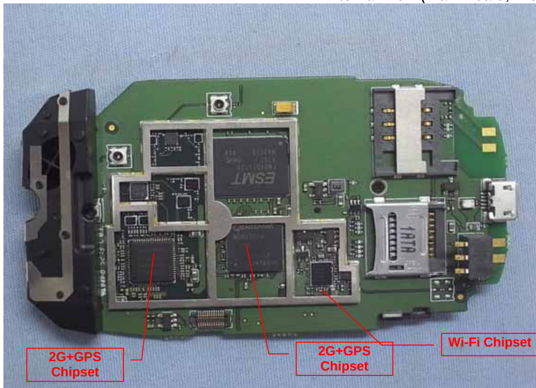
Photo 11 Internal View (Main Board, Front View)
