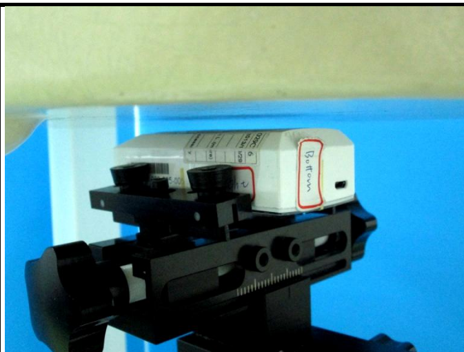
Rear Face of EUT with 0.5 cm Gap
