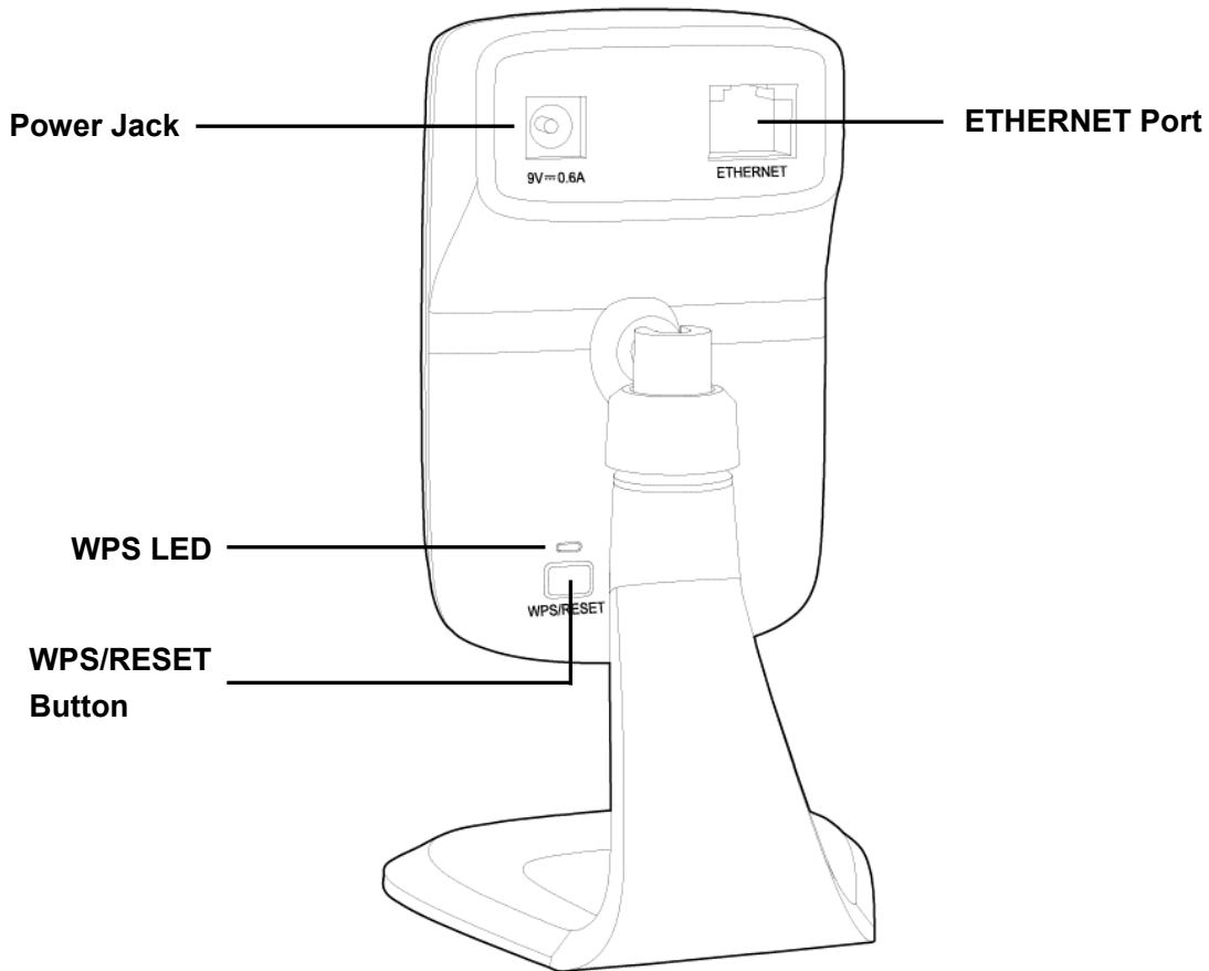
Figure 2-2 Rear Panel
