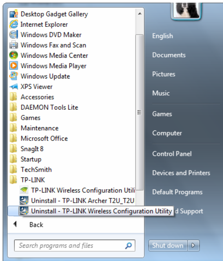
Figure 6-1 Uninstall Utility
