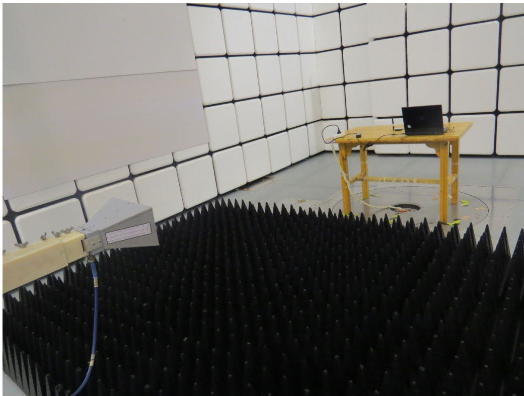
b: Above 1GHz Radiated Emission Test Setup
