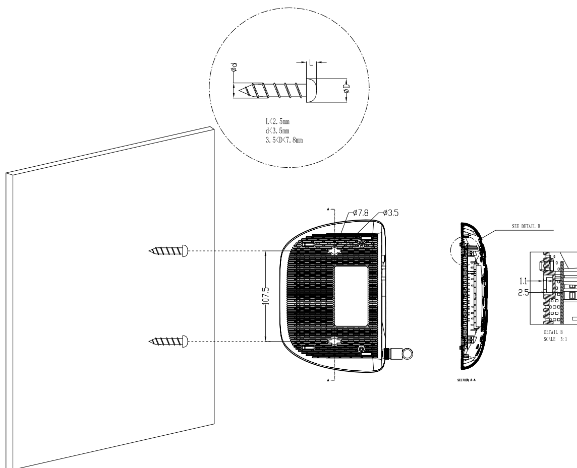
Figure 2-3 Wall-mount Install
