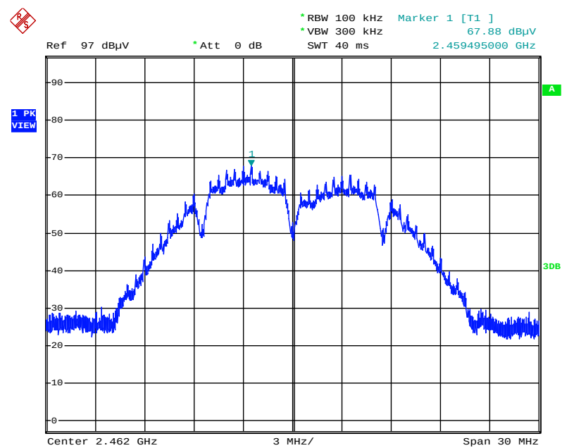
Plot on Configuration IEEE 802.11b / Reference Level
