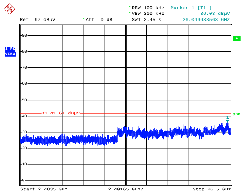
Plot on Configuration IEEE 802.11n MCS0 HT40 / CH 3 / 2483.5MHz~26500MHz (down 30dBc)
