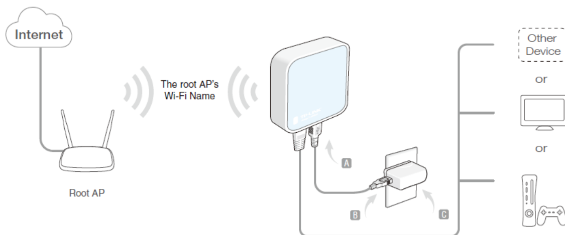
Figure 2-5 Hardware Installation of the TL-WR802N in Client Mode
