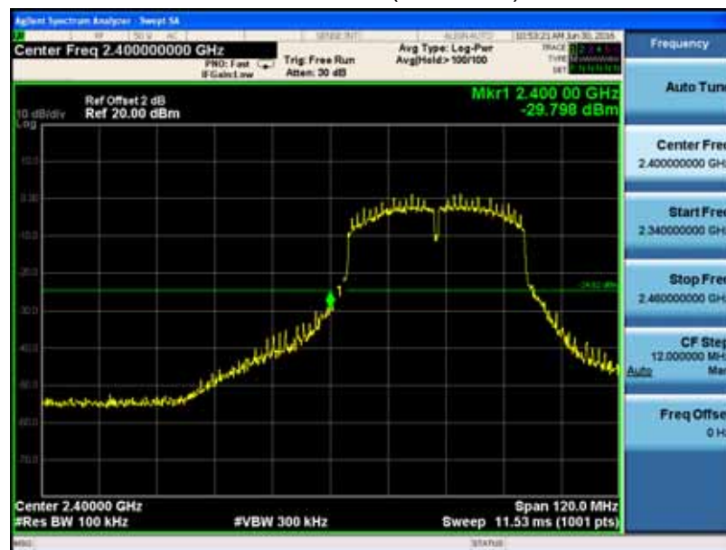
Mode 4 CH03(2422MHz)
