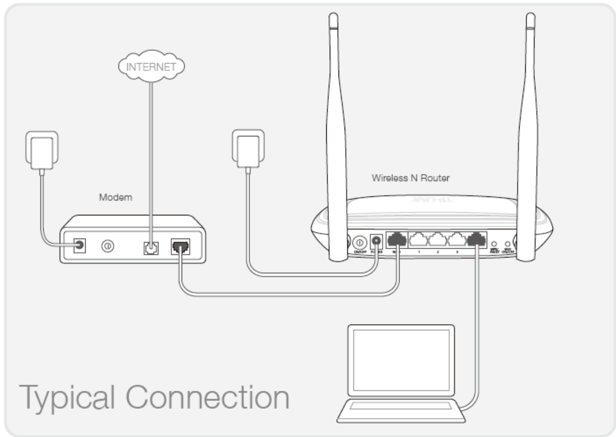
Figure 2-1 Hardware Installation of the TL-WR841ND 300Mbps Wireless N Router
