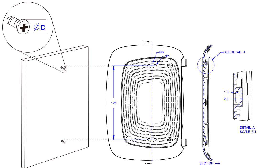
Figure 2-3 Wall-mount Install
