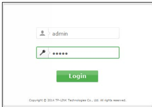
Figure 3-4 Login Windows
