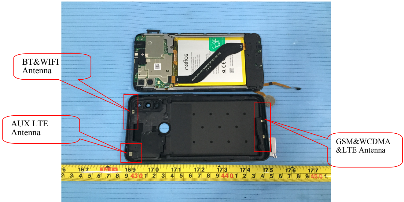
EUT – Cover off View 1
