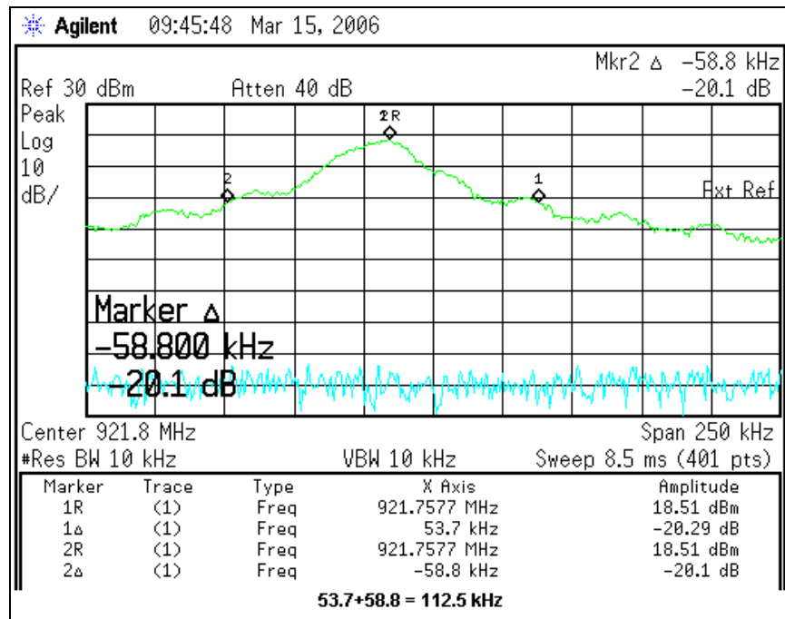
Figure 6.7.4-3: 20dB Bandwidth – High Channel
