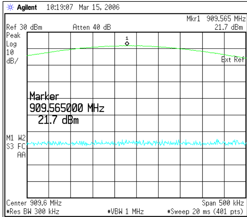
Figure 6.6-1: Output Power – Low Channel
