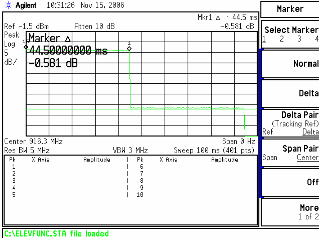
Figure 6.7.3-1: Channel Dwell Time
