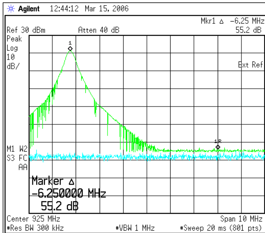
Figure 6.8.1-2: Upper Band-Edge
