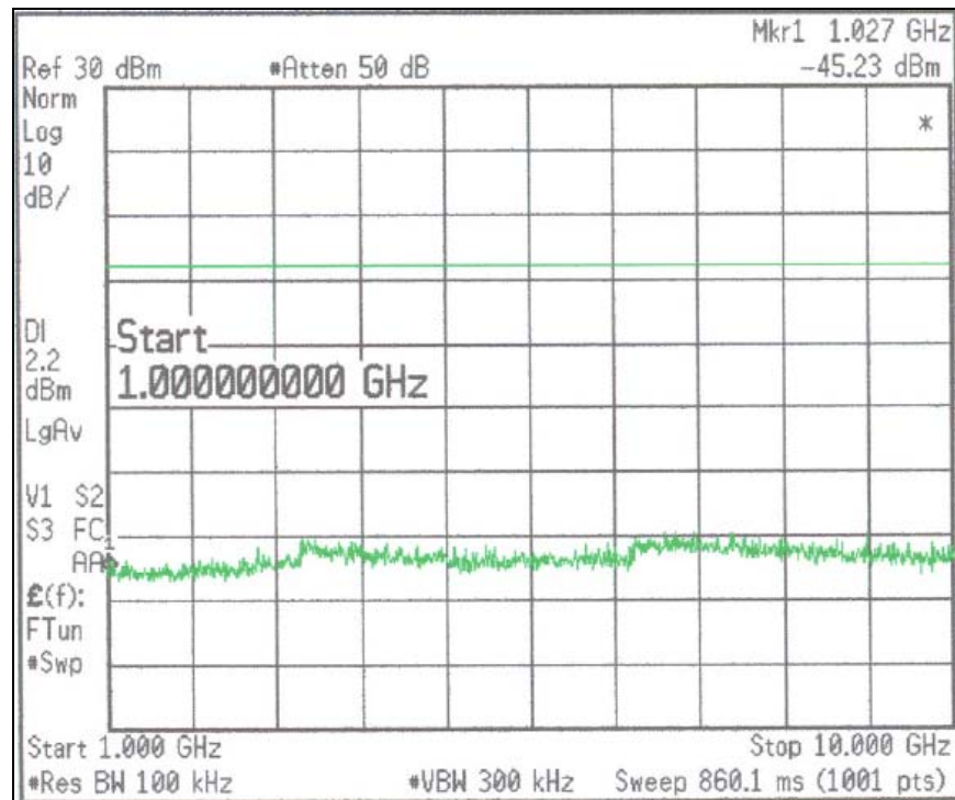
Figure 6.8.2-4: RF Conducted Spurious Emissions – Mid Channel
