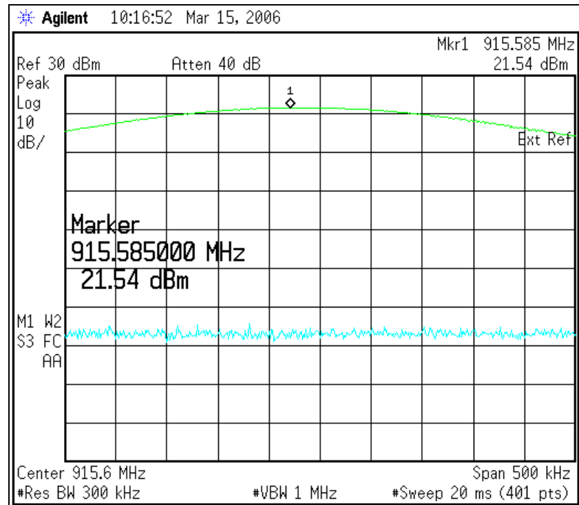
Figure 6.6-2: Output Power – Mid Channel
