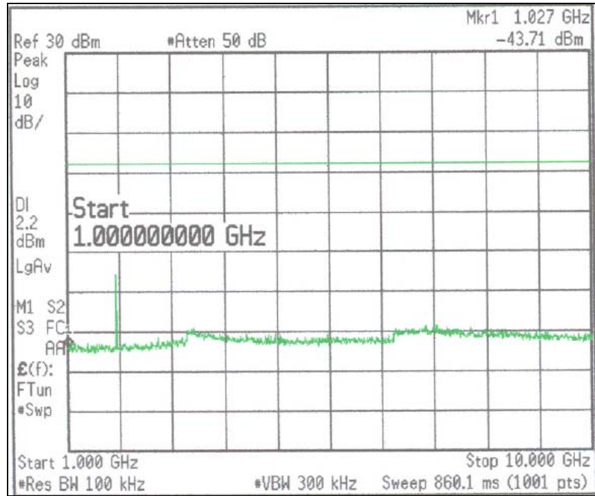
Figure 6.8.2-6: RF Conducted Spurious Emissions – High Channel
