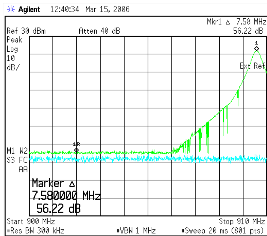
Figure 6.8.1-1: Lower Band-Edge
