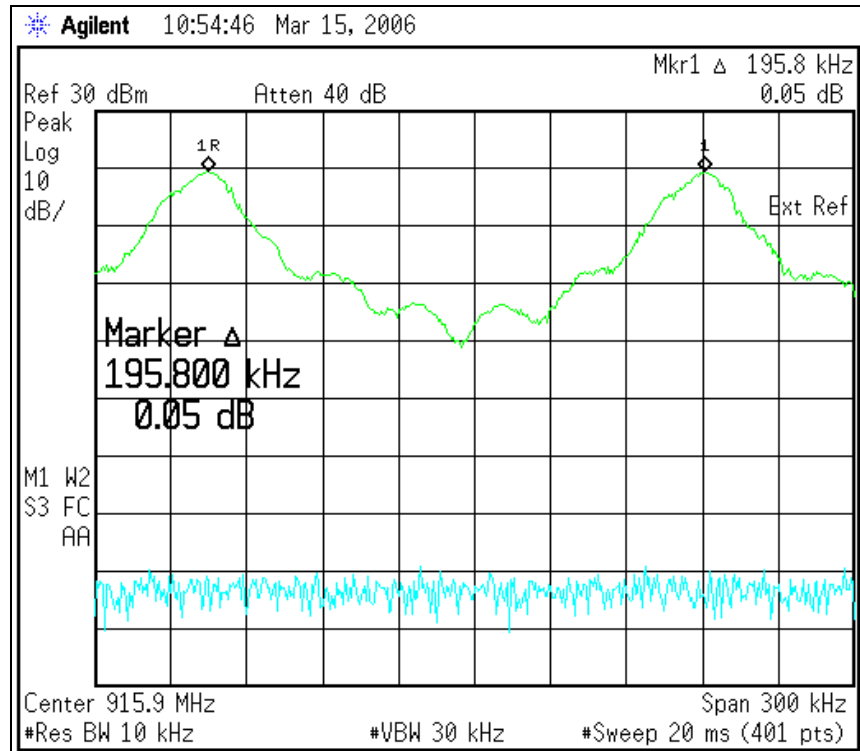
Figure 6.7.1-1: Carrier Frequency Separation
