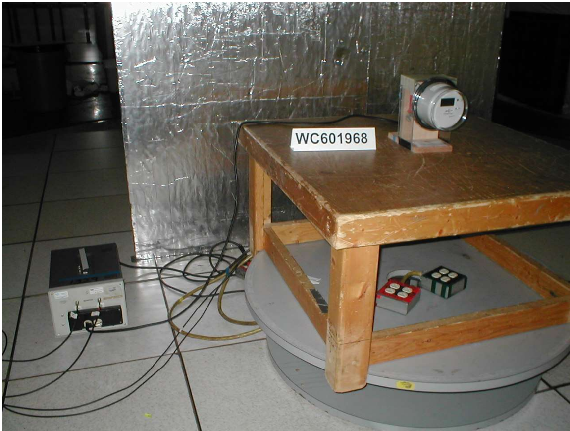
Figure 3: Conducted Emissions Setup
