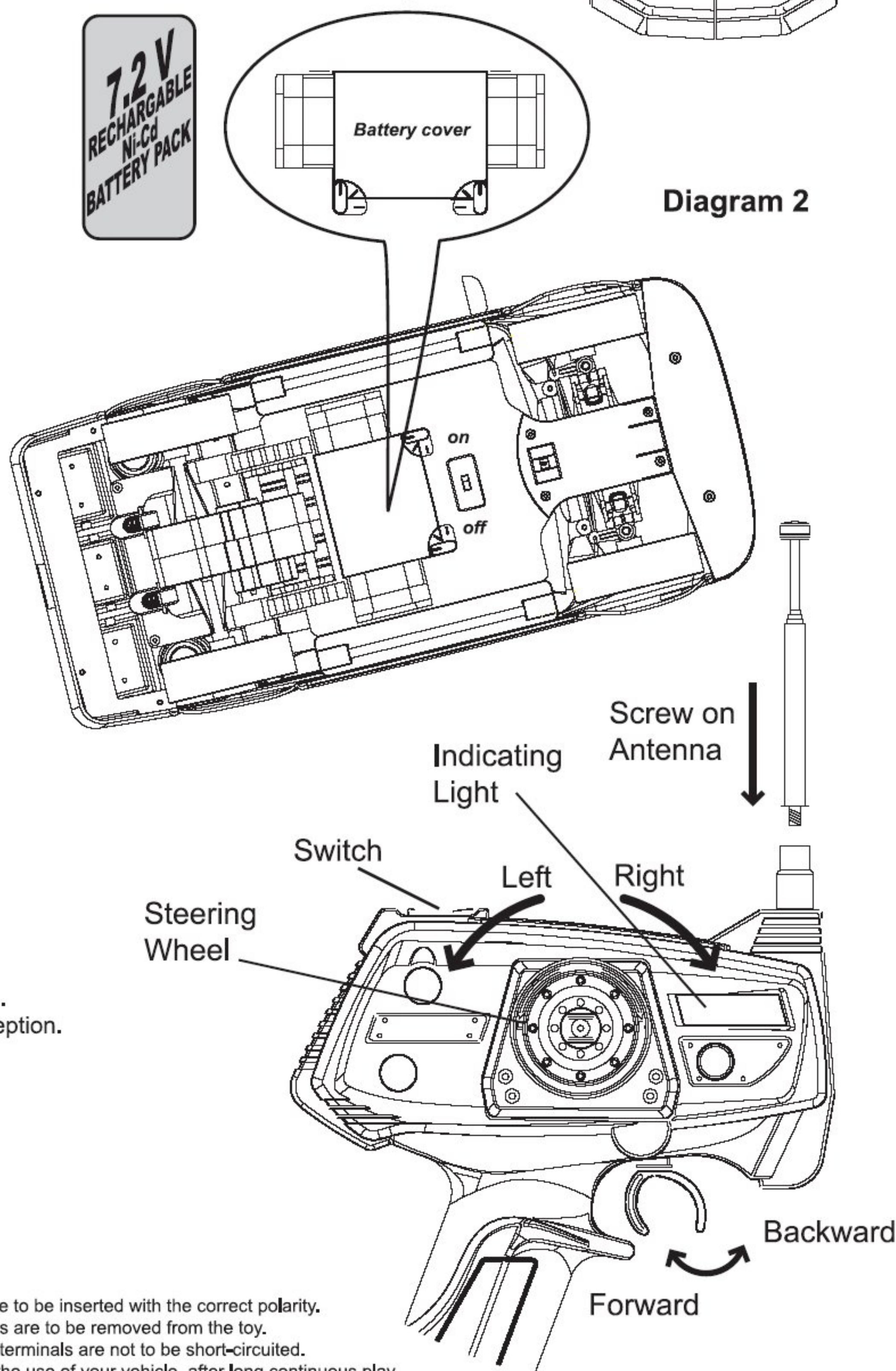
Battery Pack
