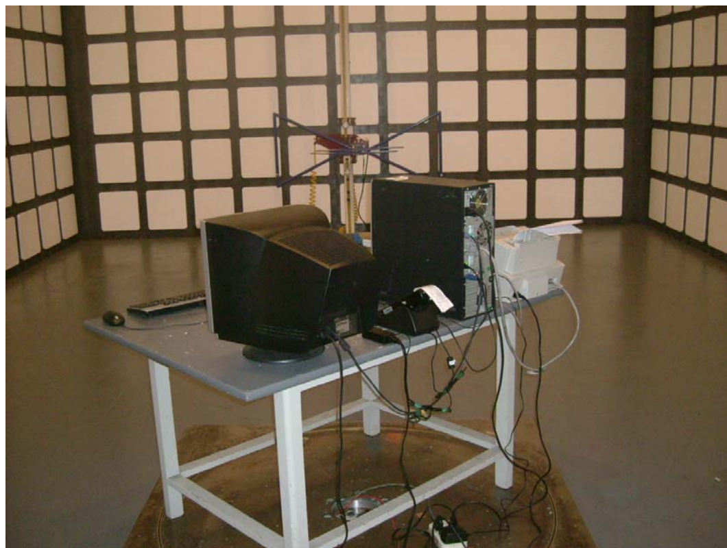
SETUP WITH MAXIMUM DETECTED EMISSION AT HORIZONTAL POLARIZATION (WITH CHARGER CRADLE)
