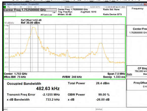
OBW_Band4_5MHz_16QAM_RB1_0_CH20375
