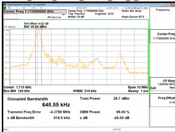
OBW_Band4_10MHz_16QAM_RB1_0_CH20175
