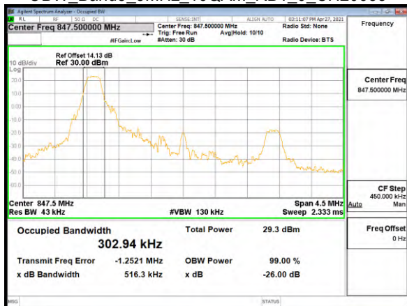
OBW_Band5_3MHz_16QAM_RB1_0_CH20635
