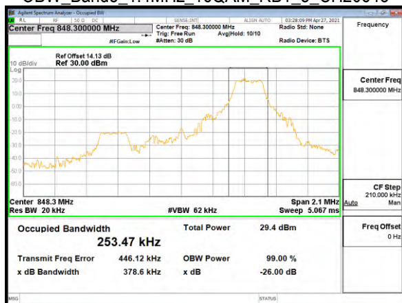
OBW_Band5_1.4MHz_16QAM_RB1_5_CH20643
