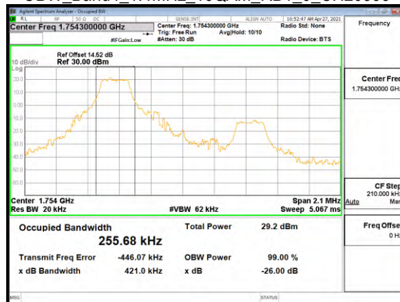
OBW_Band4_1.4MHz_16QAM_RB1_0_CH20393
