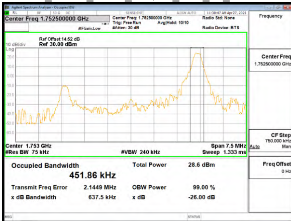
OBW_Band4_5MHz_16QAM_RB1_24_CH20375
