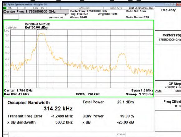
OBW_Band4_3MHz_16QAM_RB1_0_CH20385
