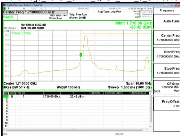
Band Edge_Band4_5MHz_QPSK_RB1_0_CH19975
