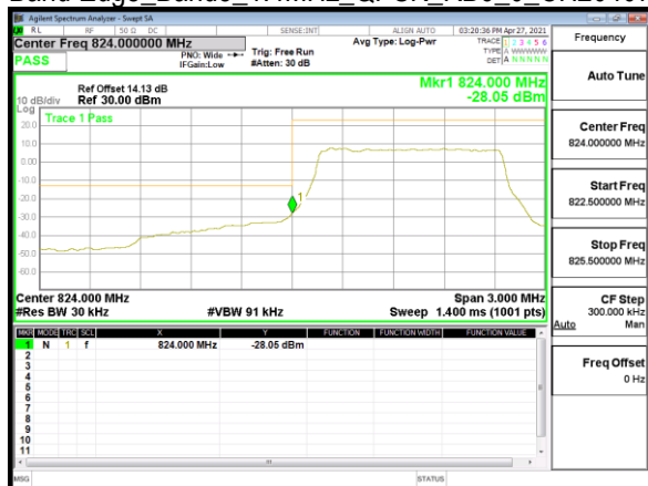
Band Edge_Band5_1.4MHz_QPSK_RB6_0_CH20407
