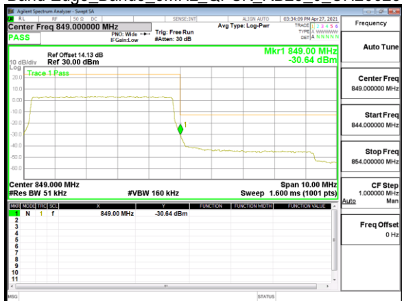
Band Edge_Band5_5MHz_QPSK_RB25_0_CH20625
