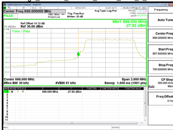
Band Edge_Band12_1.4MHz_QPSK_RB6_0_CH23173
