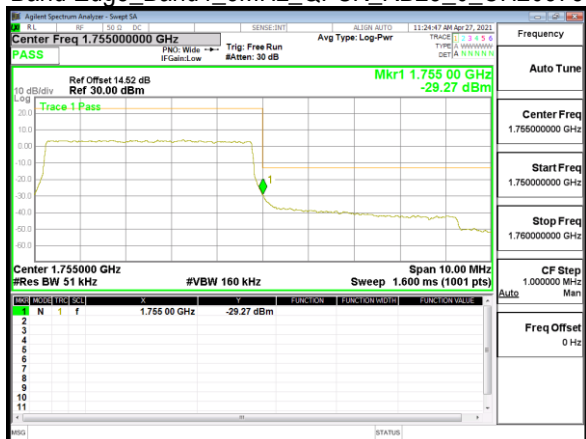
Band Edge_Band4_5MHz_QPSK_RB25_0_CH20375
