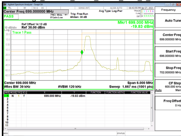
Band Edge_Band12_3MHz_QPSK_RB1_0_CH23025
