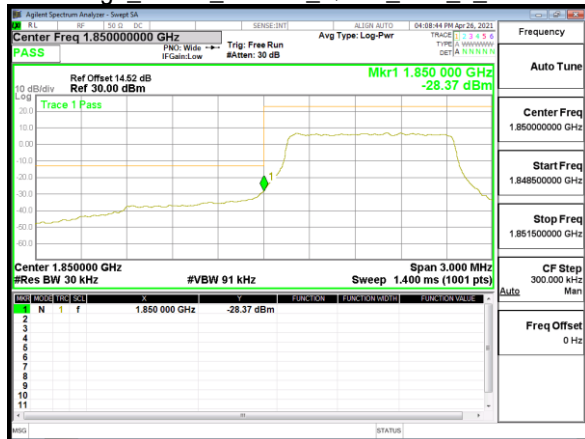
Band Edge_Band2_1.4MHz_QPSK_RB6_0_CH18607
