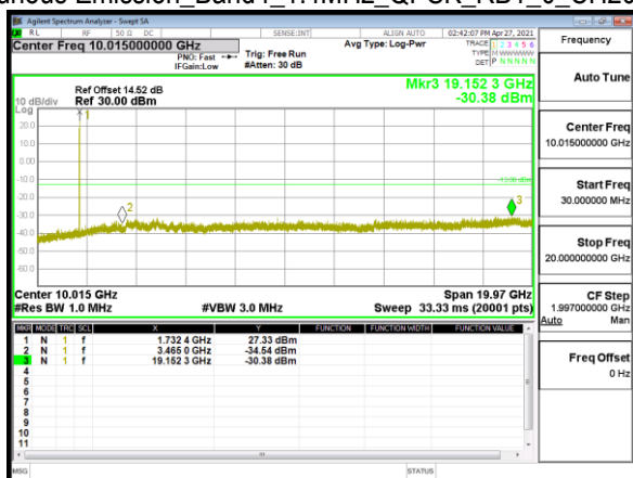
Spurious Emission_Band4_1.4MHz_QPSK_RB1_0_CH20393
