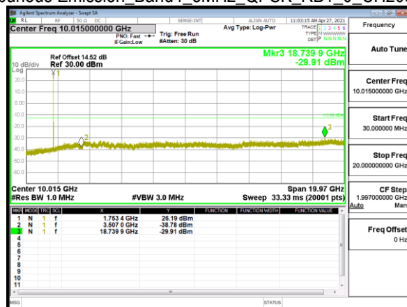
Spurious Emission_Band4_3MHz_QPSK_RB1_0_CH20385
