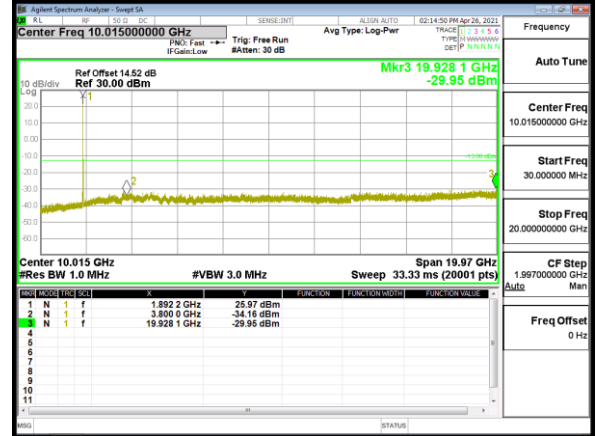
Spurious Emission_Band2_20MHz_QPSK_RB1_0_CH19100
