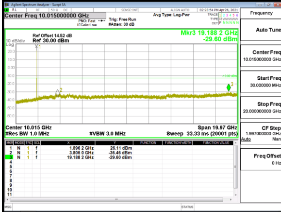
Spurious Emission_Band2_15MHz_QPSK_RB1_0_CH19125
