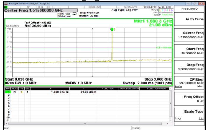
WCDMA_B2_MidCH9400-1880
