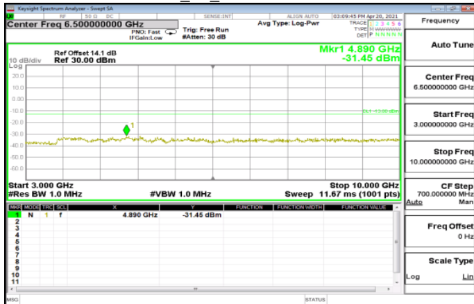
HSUPA_B5_LowCH4132-826.4
