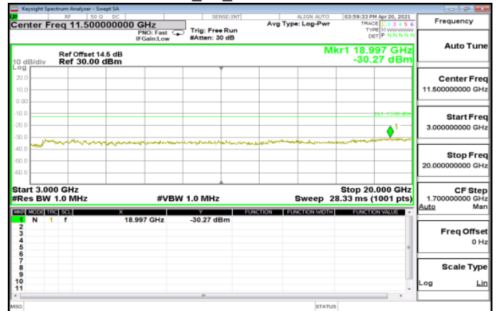
HSUPA_B2_MidCH9400-1880
