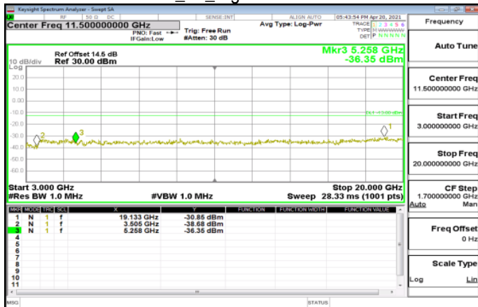
HSUPA_B4_HighCH1513-1752.6
