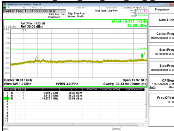
Spurious Emission_Band2_5MHz_QPSK_RB1_0_CH19175
