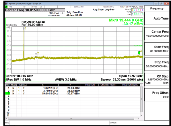
Spurious Emission_Band2_20MHz_QPSK_RB1_0_CH19100
