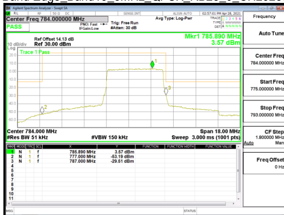
Band Edge_Band13_5MHz_QPSK_RB25_0_CH23255
