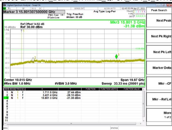
Spurious Emission_Band4_1.4MHz_QPSK_RB1_0_CH20175
