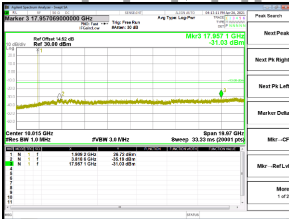
Spurious Emission_Band2_1.4MHz_QPSK_RB1_0_CH19193
