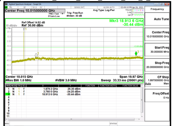
Spurious Emission_Band2_3MHz_QPSK_RB1_0_CH19185
