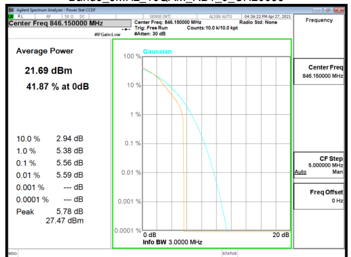
Band5_3MHz_16QAM_RB1_0_CH20635
