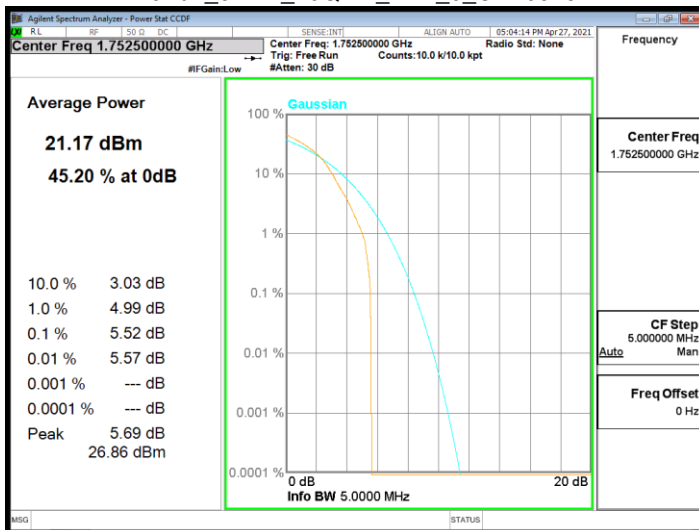
Band4_5MHz_16QAM_RB1_0_CH20375
