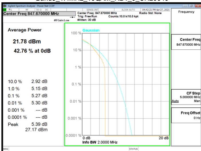
Band5_1.4MHz_16QAM_RB1_0_CH20643
