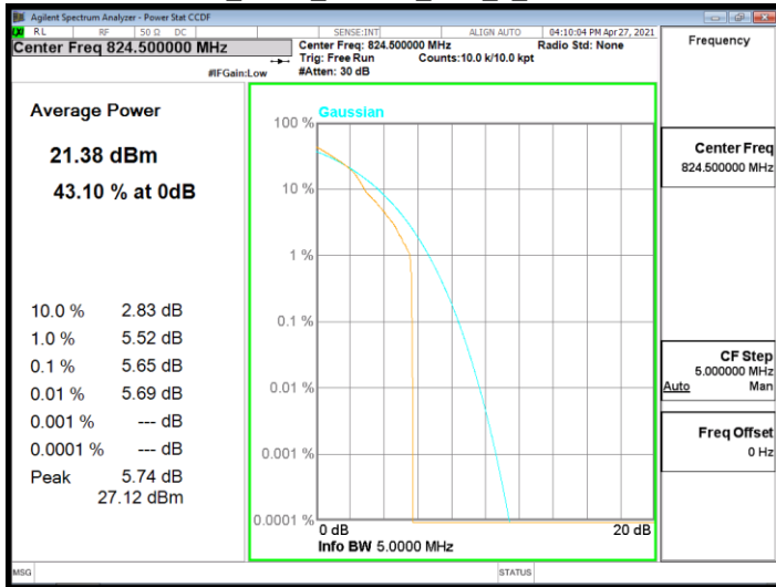
Band5_5MHz_16QAM_RB1_0_CH20525
