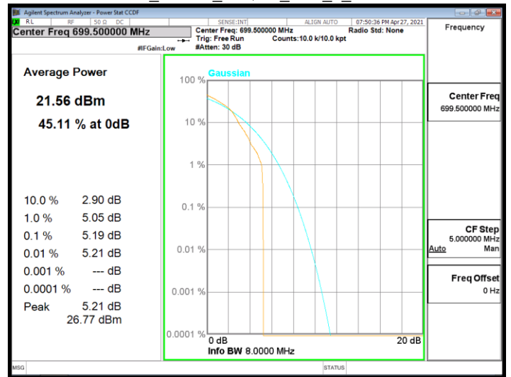
Band12_10MHz_16QAM_RB1_0_CH23095
