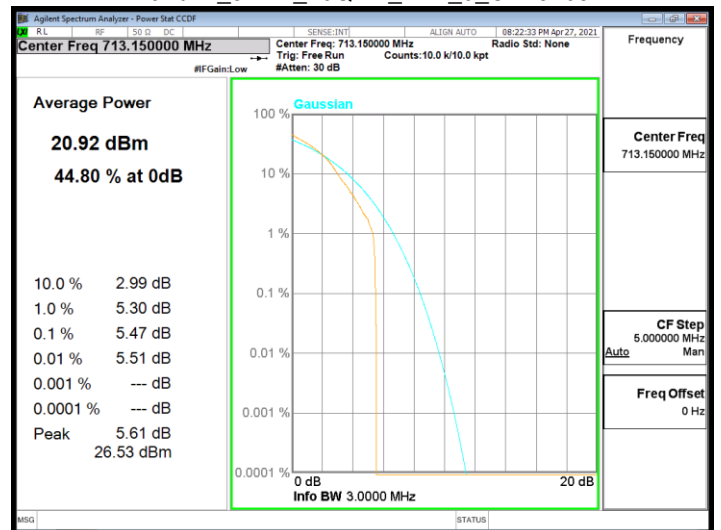
Band12_3MHz_16QAM_RB1_0_CH23165
