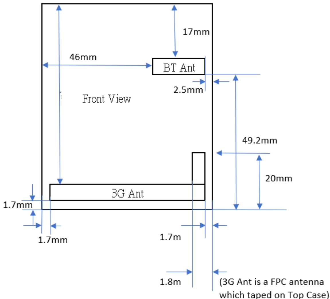
Fig.7 Antenna location
