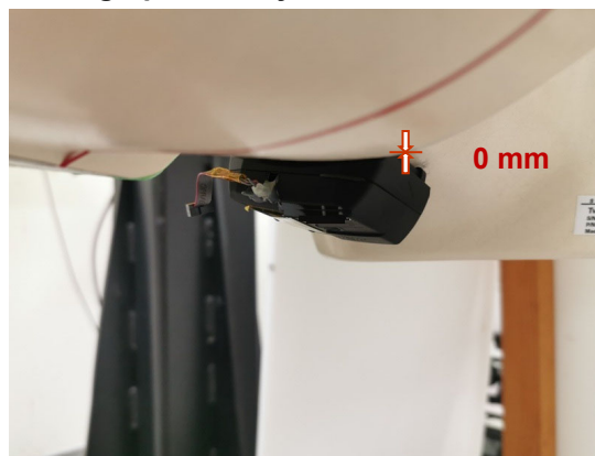
Photograph 4. Product specific 10-g SAR, Back Surface, 0mm
