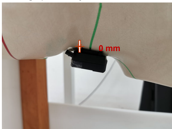
Photograph 3. Product specific 10-g SAR, Back Surface, 0mm
