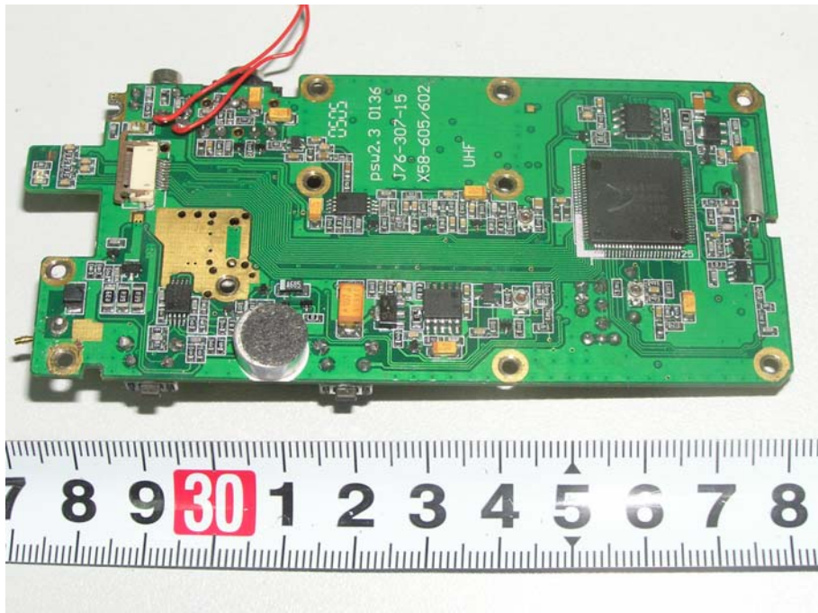
EUT – Mainboard View (2)
