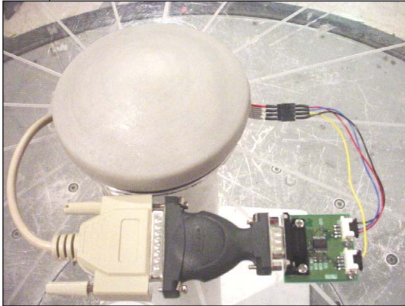
Top view of the EUT (Gray Circular Footswitch)
