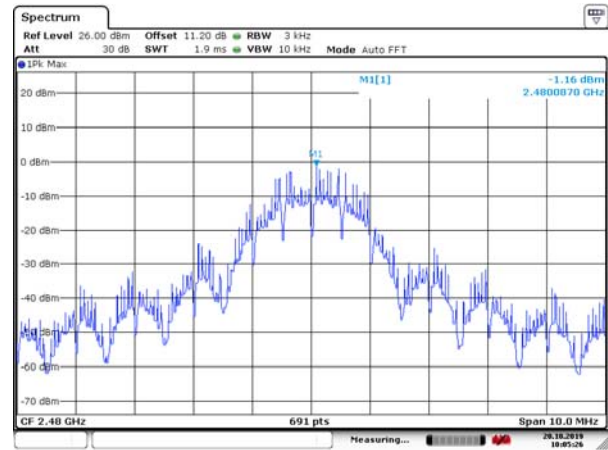
High Channel 2480 MHz
