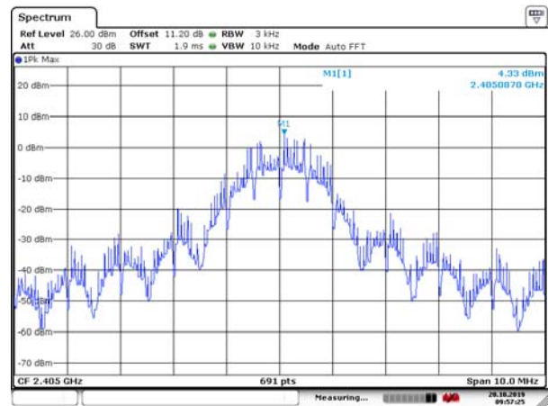
Low Channel 2405 MHz
