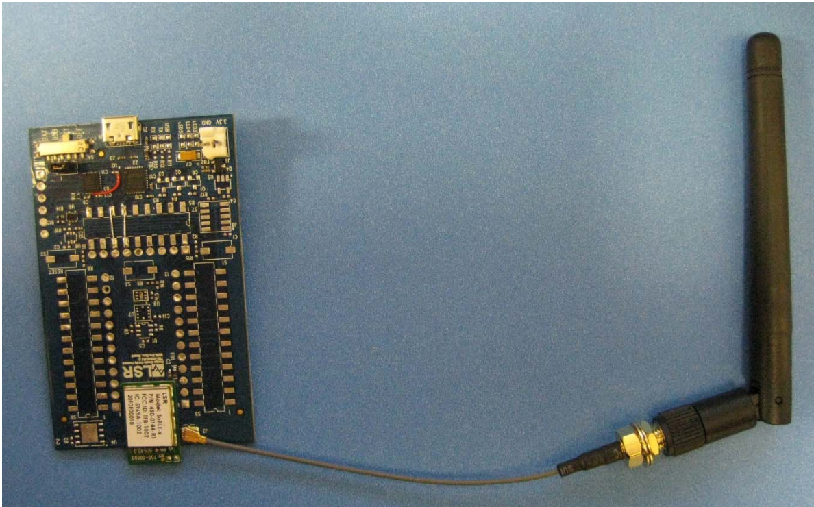
Module with dipole antenna attached
