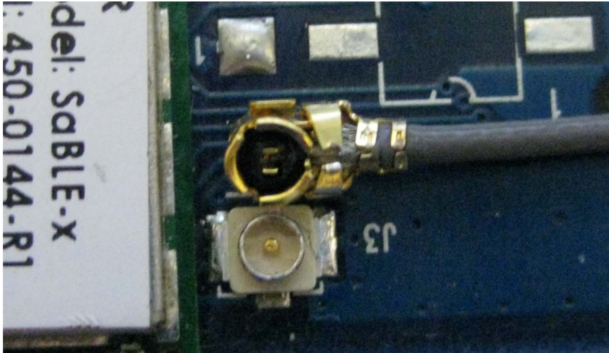
u.fl cable connection (Picture 1)
