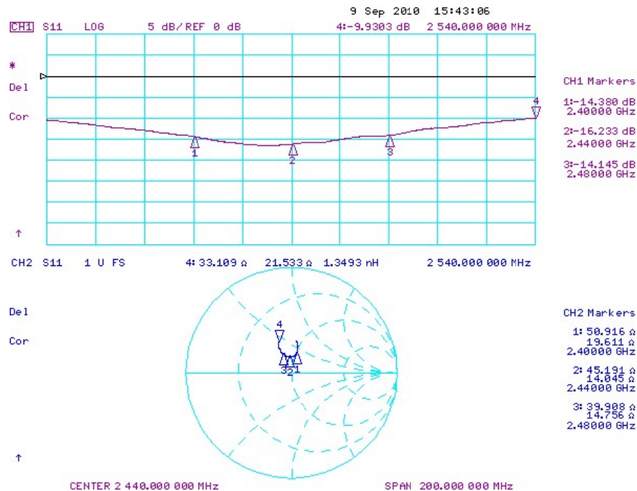
Figure 2 Reflection Parameters for Folded Configuration (S11)
