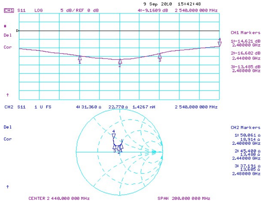
Figure 1 Reflection Parameters for Extended Configuration (S11)
