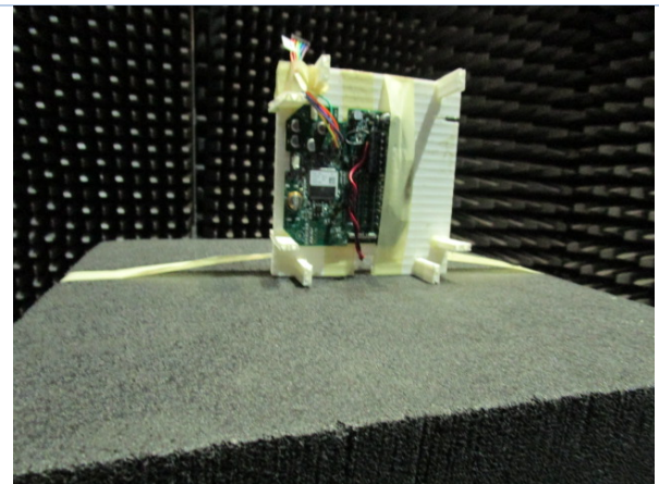
EUT Vertical Orientation
