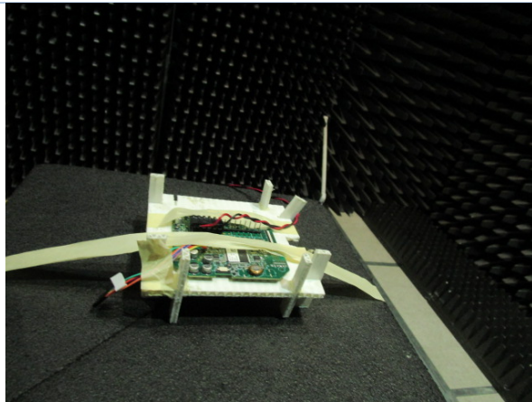
EUT Flat Orientation
