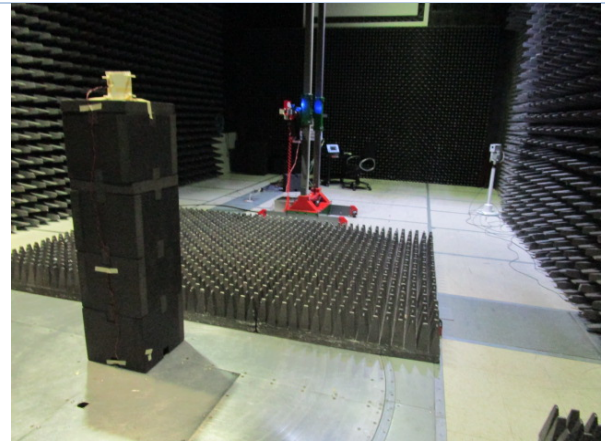
Radiated Emissions Setup
