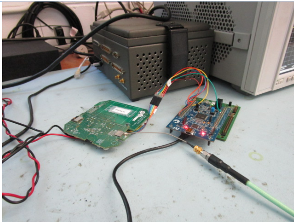
BT Conducted Radio Testing
