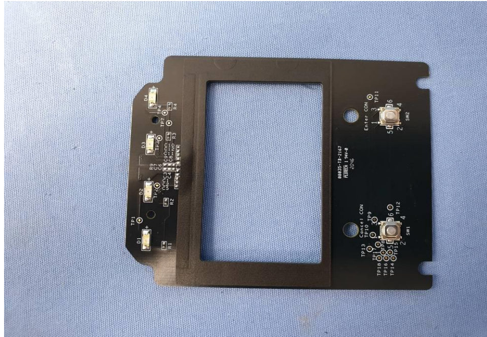
EUT Photo (29)
