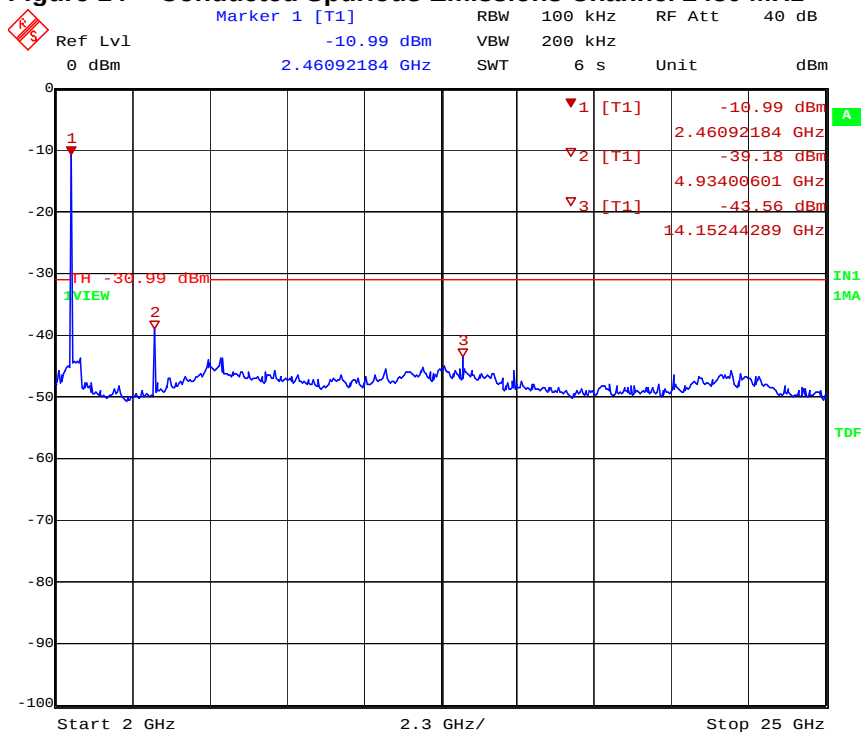
Figure 14 Conducted Spurious Emissions Channel 2480 MHz
