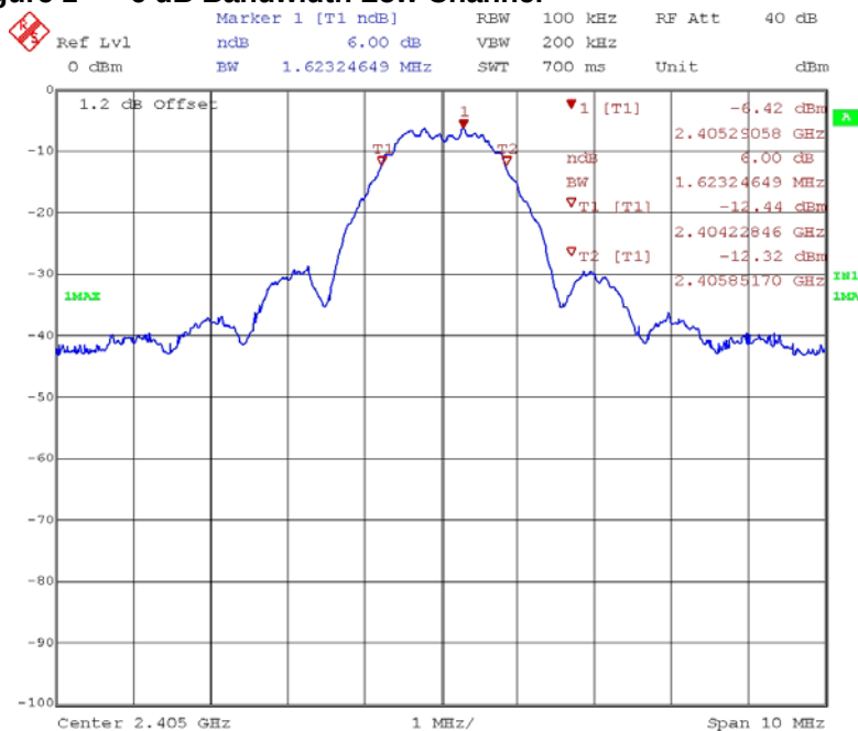
Figure 1 6 dB Bandwidth Low Channel
