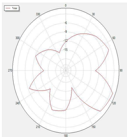
2480P0 Total
