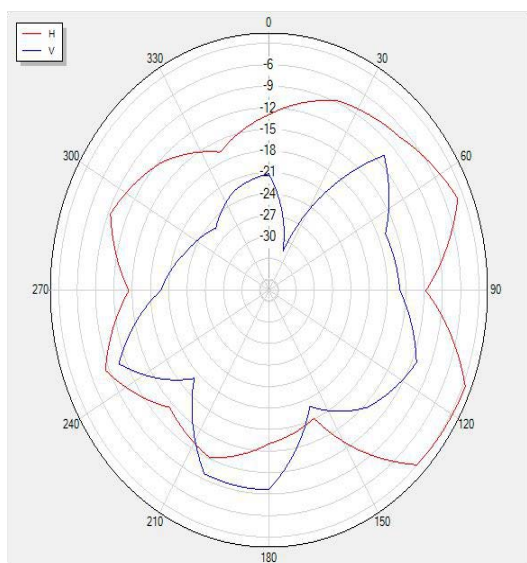
2480P0 Polar
