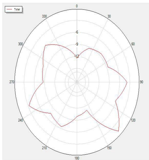
2500P90 Total
