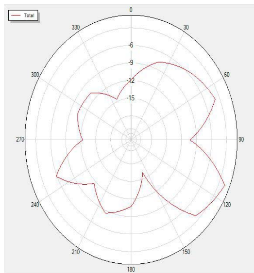
2420P0 Total
