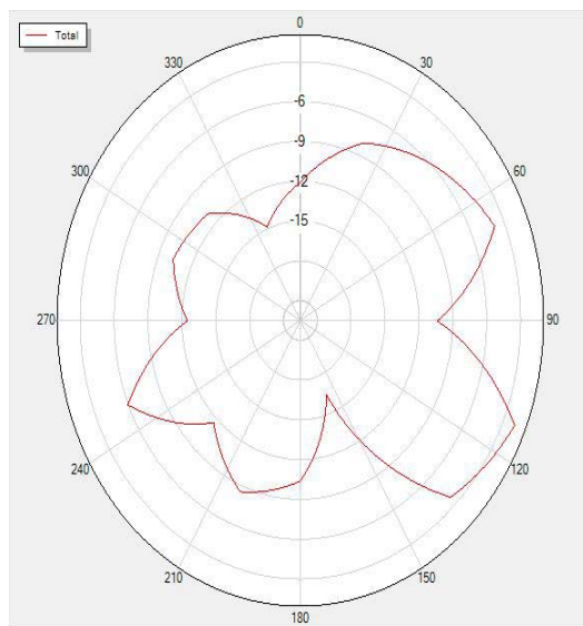
2430P0 Total
