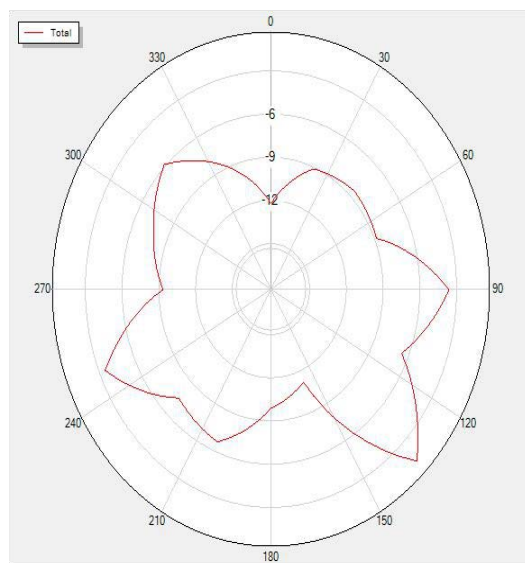
2490P90 Total
