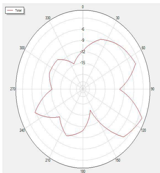
2410P0 Total
