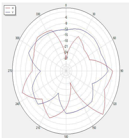
2450P90 Polar
