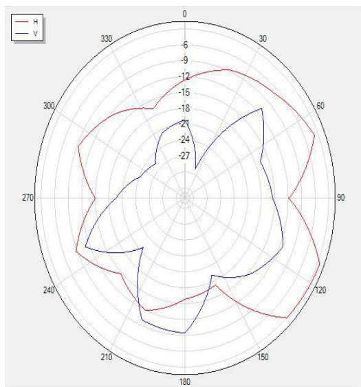
2490P0 Polar
