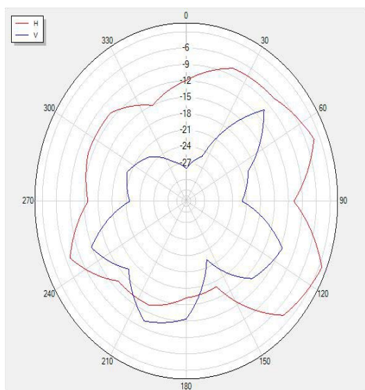
2410P0 Polar
