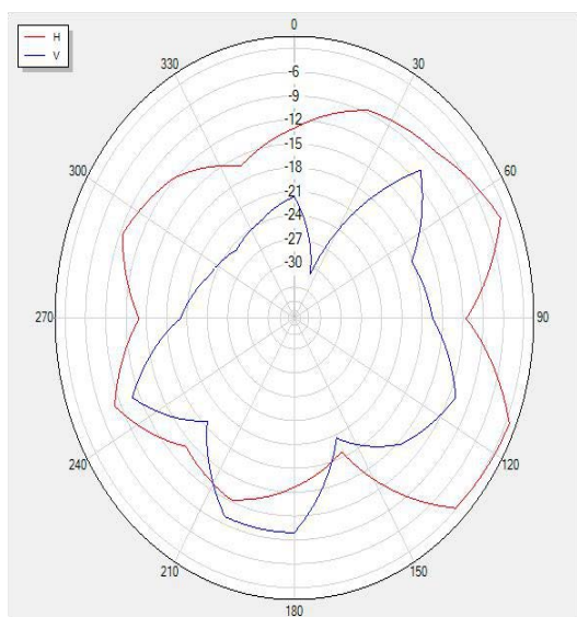
2470P0 Polar
