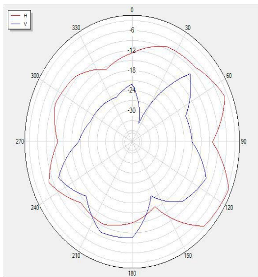
2450P0 Polar
