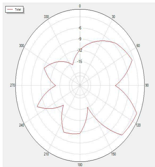
2490P0 Total
