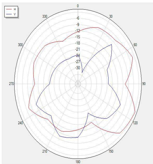
2430P0 Polar
