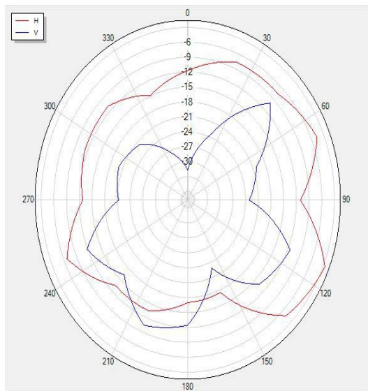
2400P0 Polar
