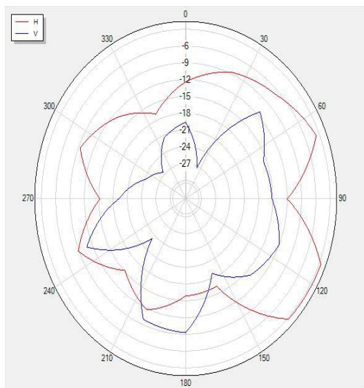
2500P0 Polar
