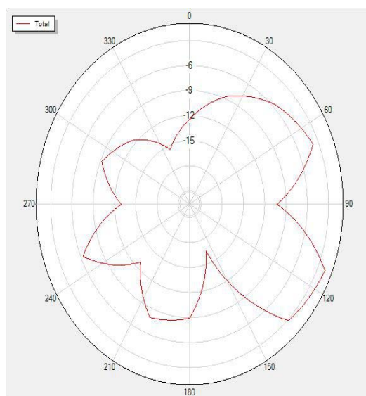
2470P0 Total
