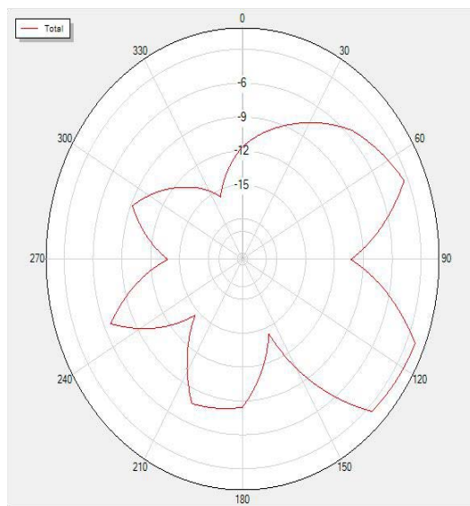
2500P0 Total
