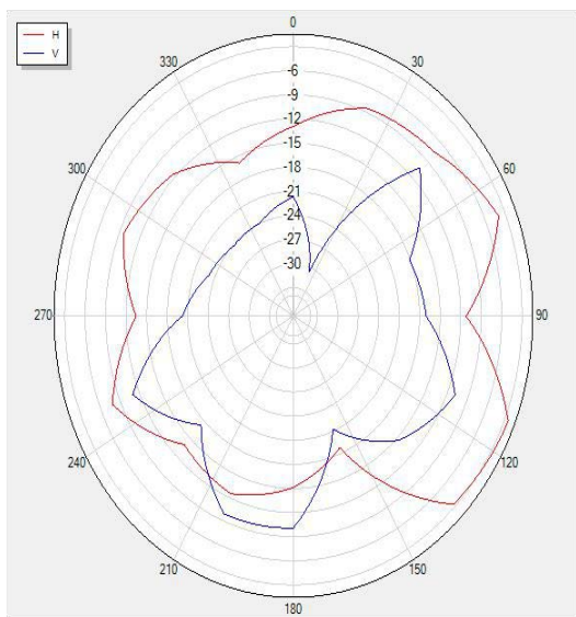
2460P0 Polar
