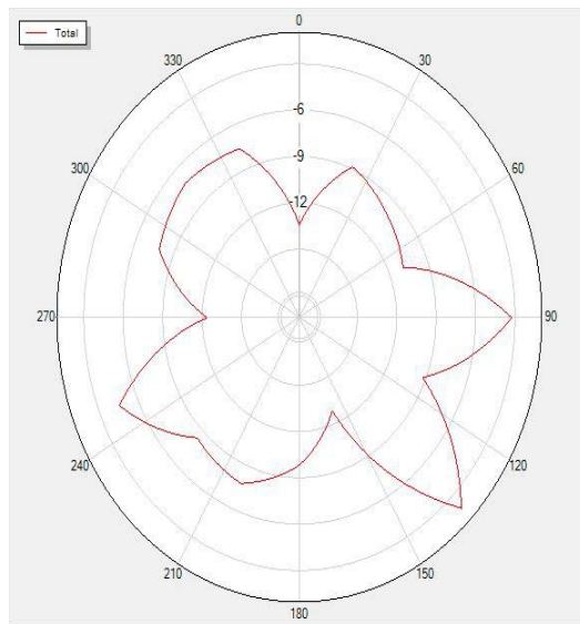
2420P90 Total
