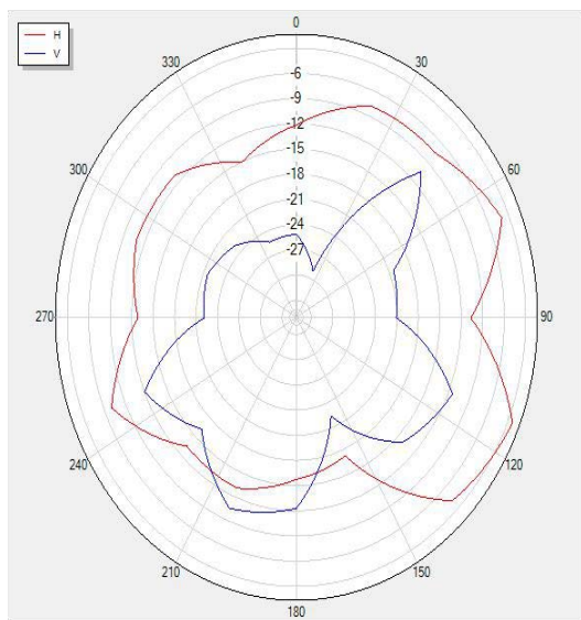
2420P0 Polar
