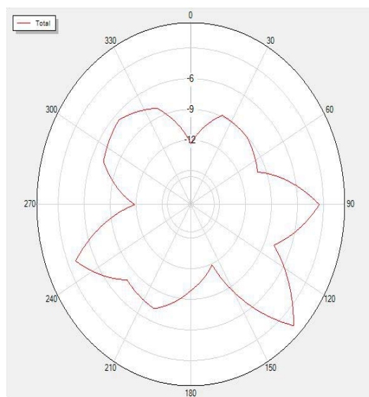
2450P90 Total
