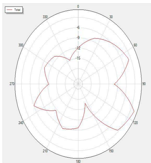
2440P0 Total
