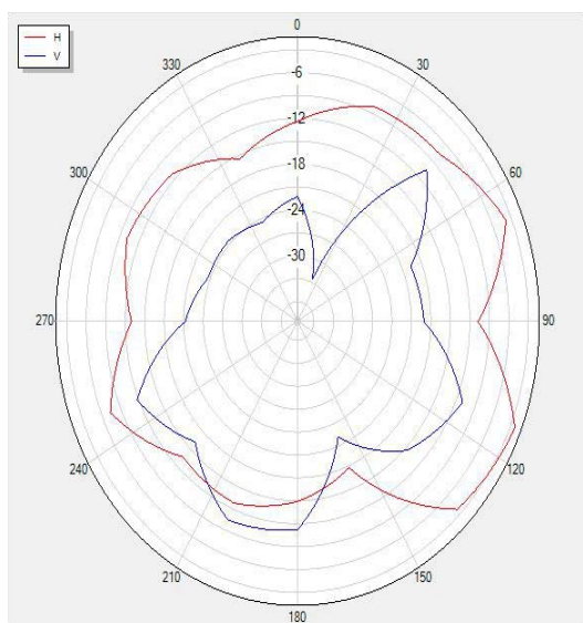
2440P0 Polar
