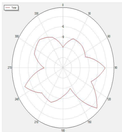
2460P90 Total
