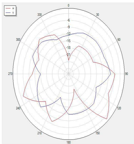
2490P90 Polar
