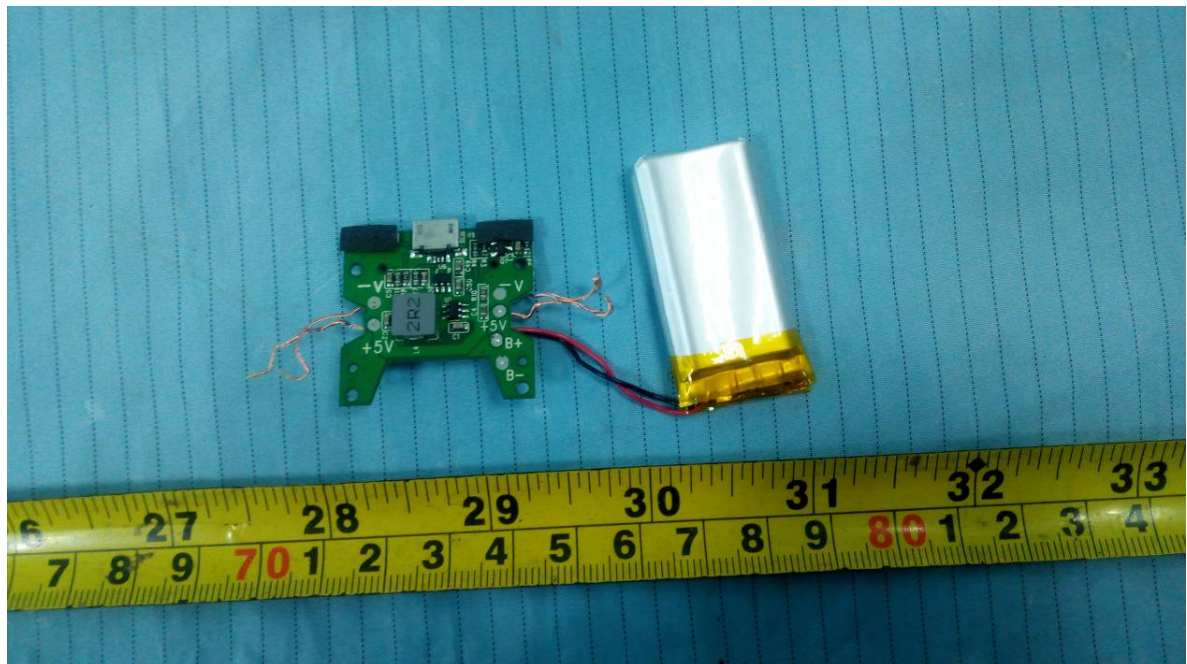
EUT – Main Board & Battery Bottom View
