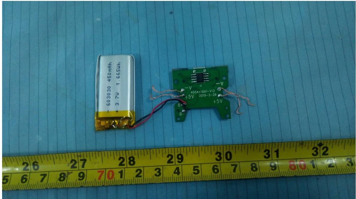
EUT – Main Board & Battery Top View
