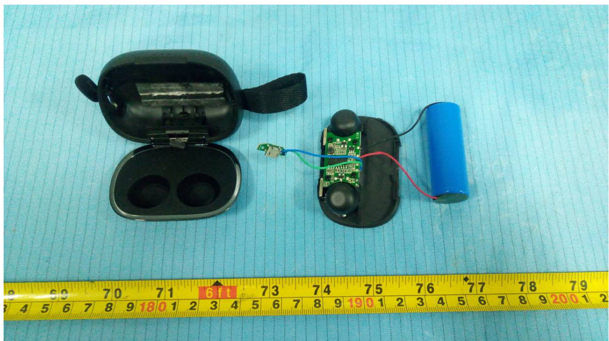
EUT – Charger Cover off View 1
