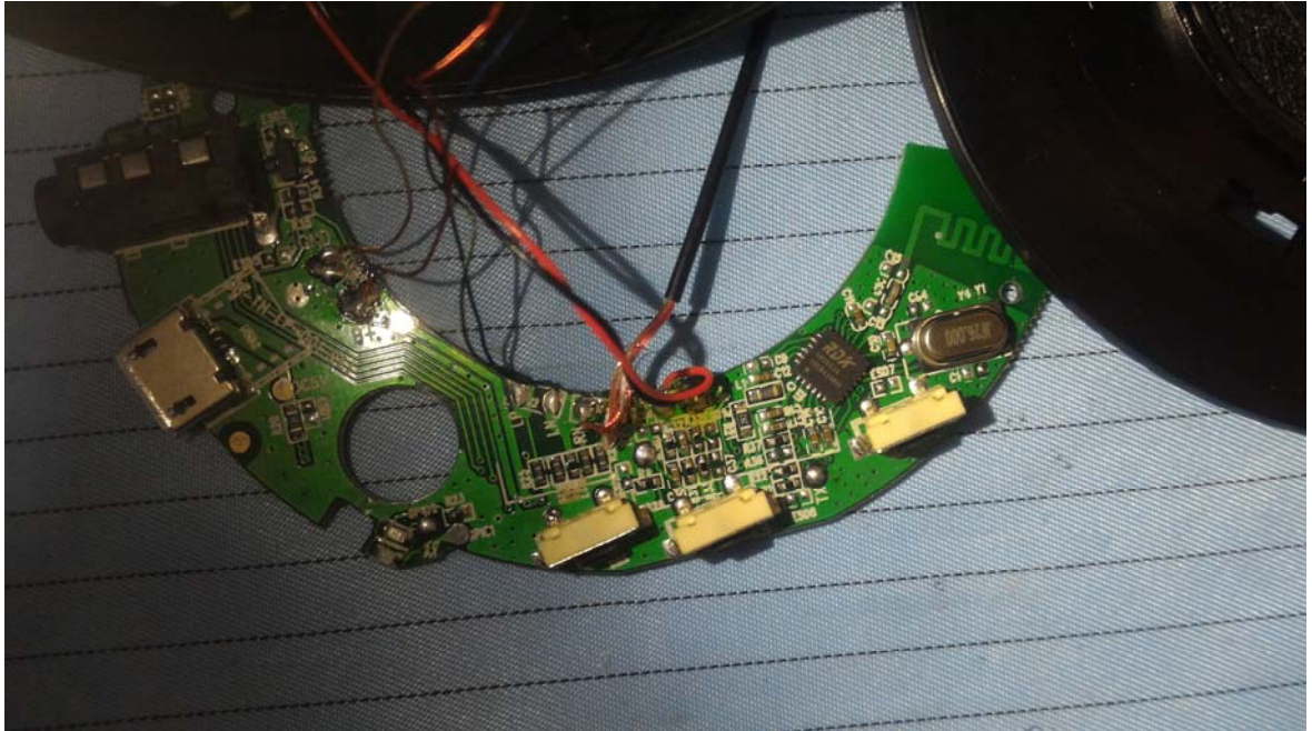
EUT – Main Chip View
