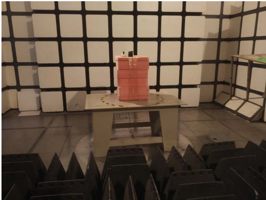
Radiated Emissions- Side View (Above 1 GHz)
