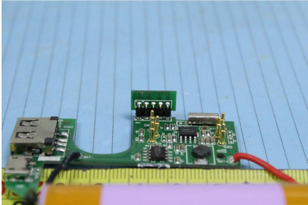
EUT – Main Board Rear View (Portable Charging Case)
