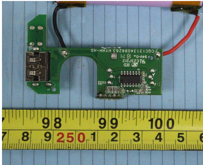
EUT – Main Board Bottom View (Portable Charging Case)
