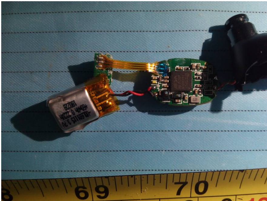
EUT – Main Chip View (Earbud)
