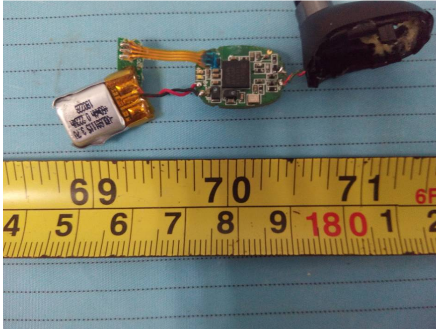
EUT – Main Board Bottom View (Earbud)
