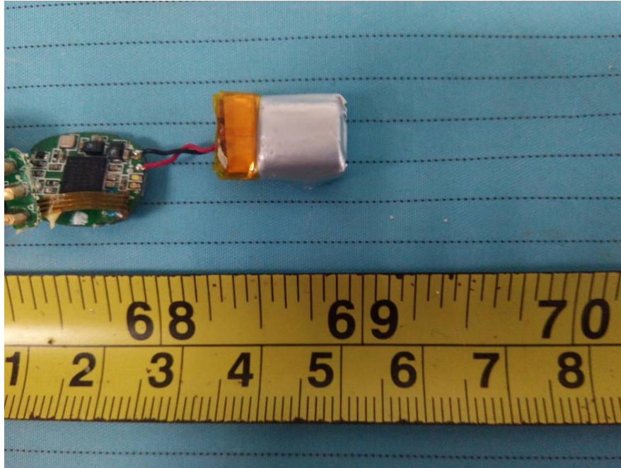
EUT – Battery Bottom View (Earbud)
