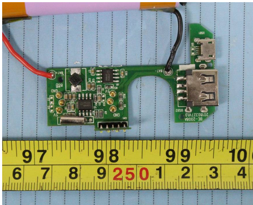
EUT – Main Board Top View (Portable Charging Case)
