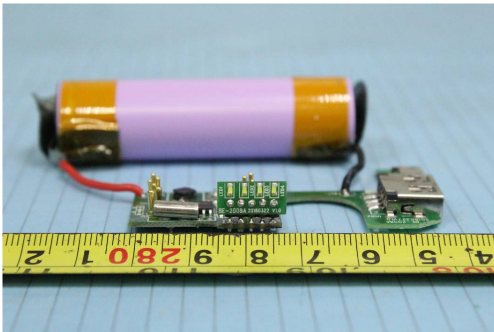
EUT – Main Board Front View (Portable Charging Case)
