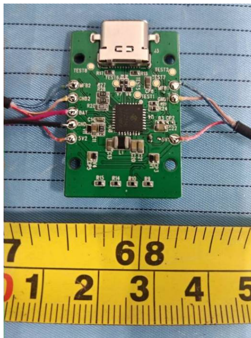
Charger Case Main Board Top View
