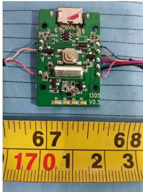
Charger Case Main Board Bottom View
