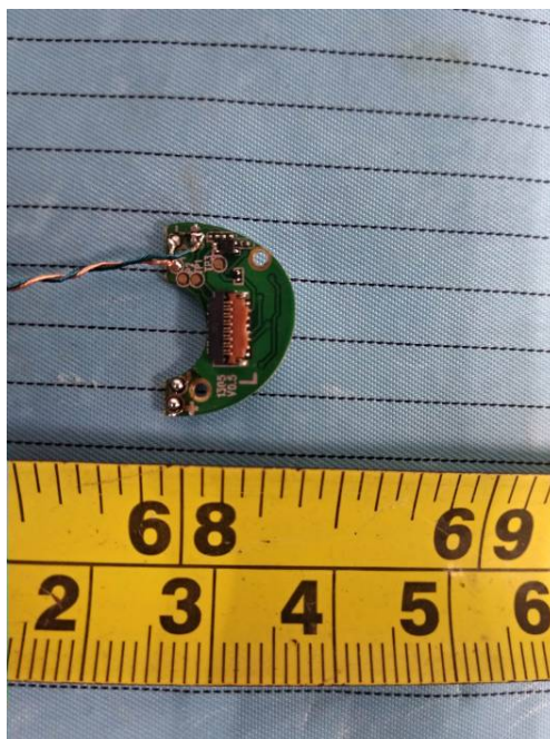
EUT – Main Board Top View
