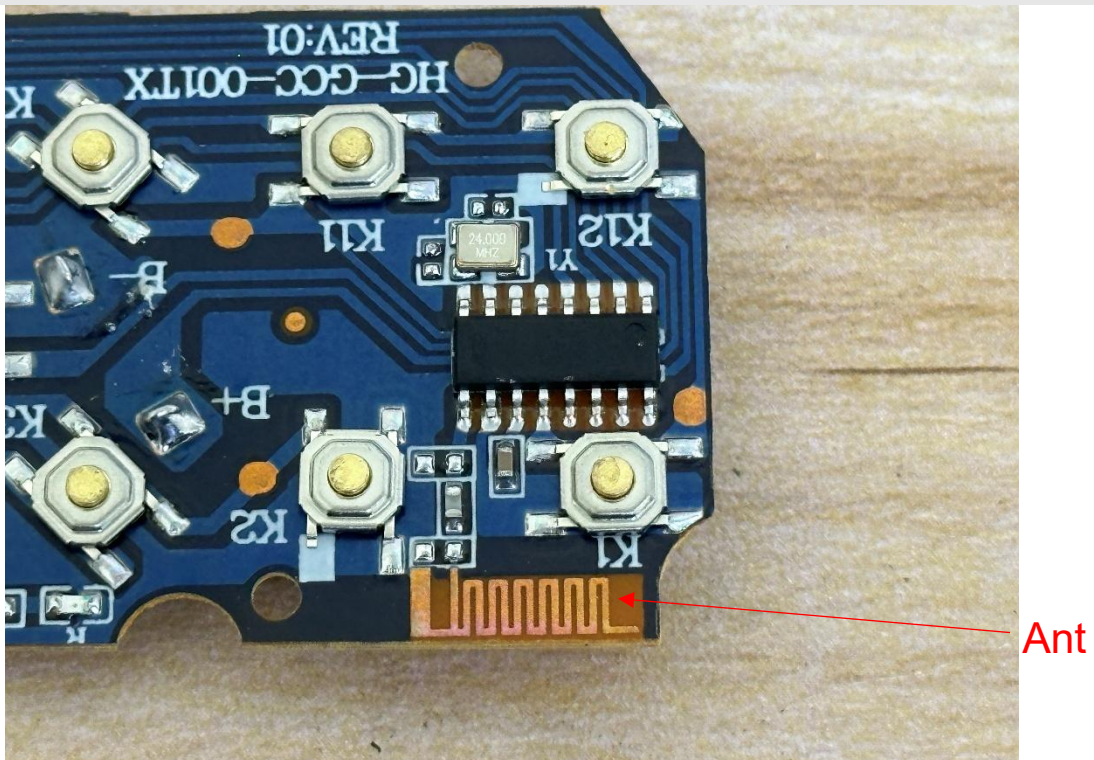
Internal View of EUT-6
