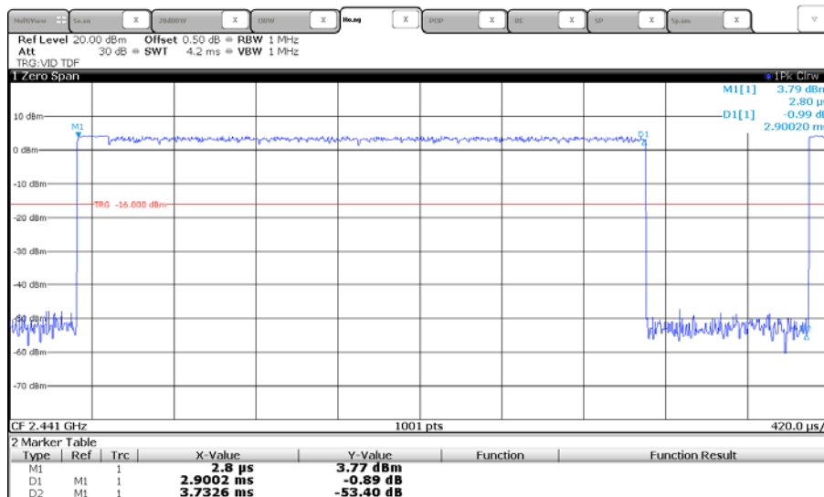
Middle Channel (2 441 MHz)
