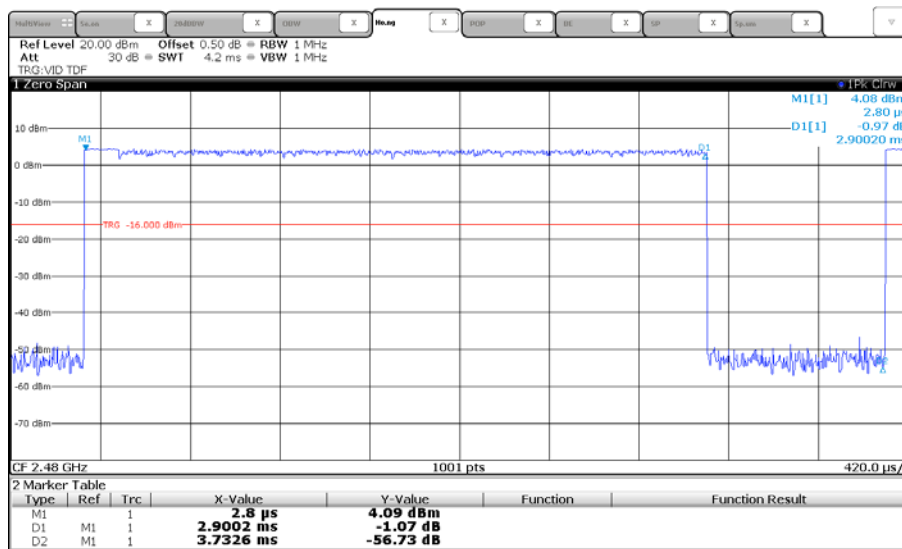
Highest Channel (2 480 MHz)
