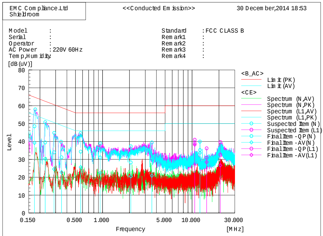
Figure4. plot of Conducted Emission
