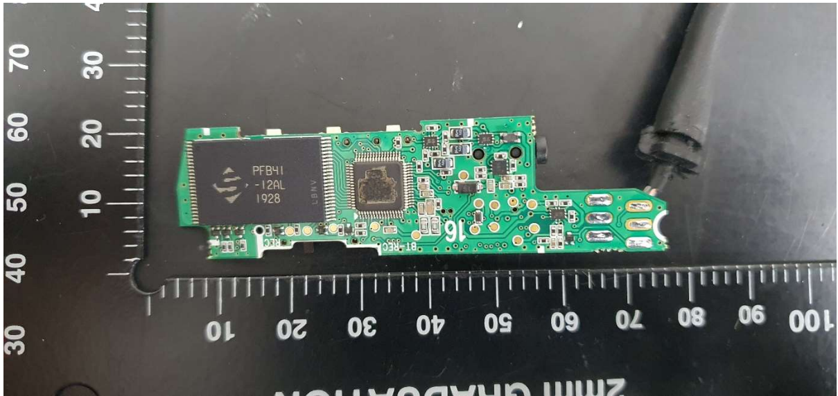
Sub Board 1 (Front)
