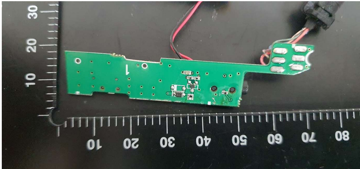
Sub Board 2 (rear)
