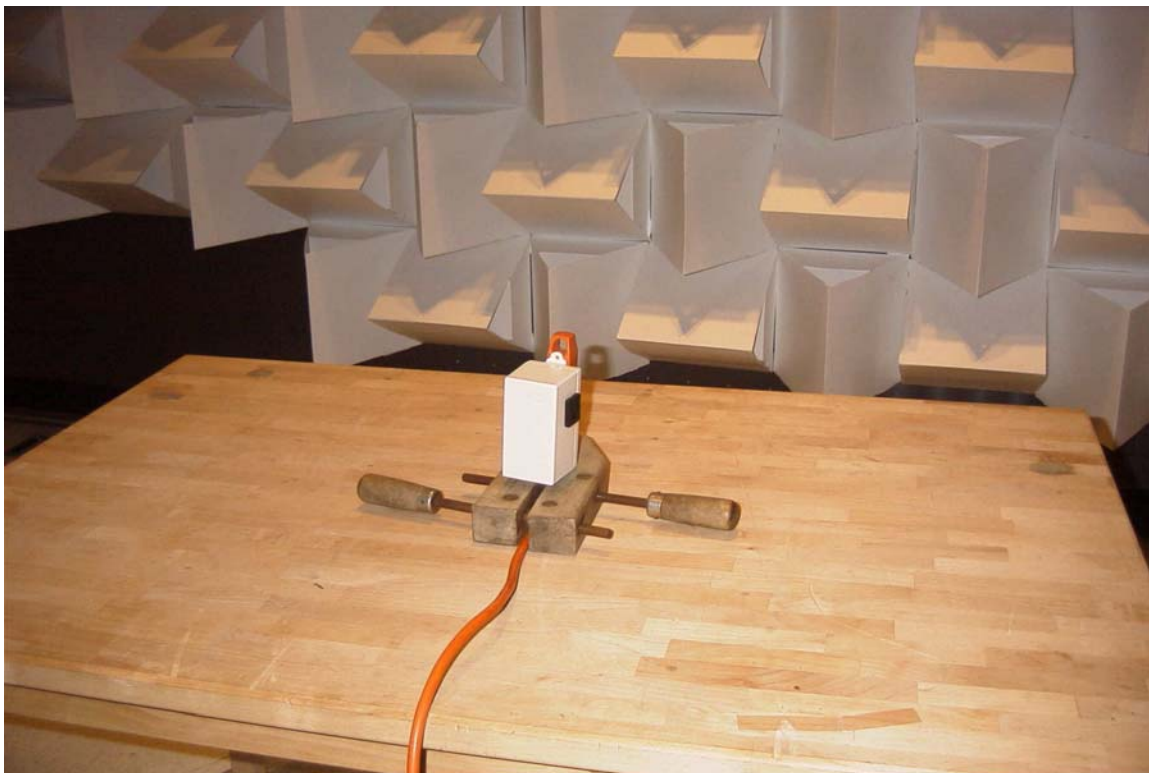
RADIATED EMISSIONS TEST SET UP PHOTO
