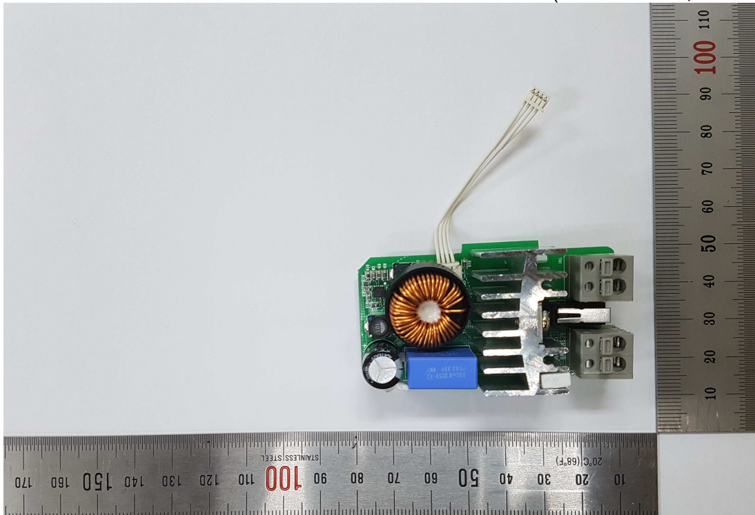
Figure 11 Internal View (Power Board, Front View)
