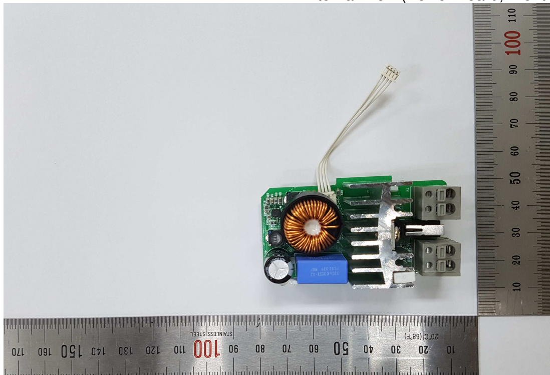
Figure 18 Internal View (Power Board, Front View)
