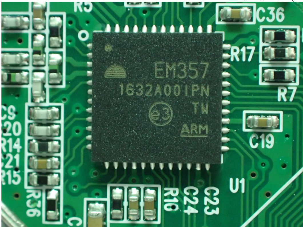
Figure 8 Internal View (RF Chip)
