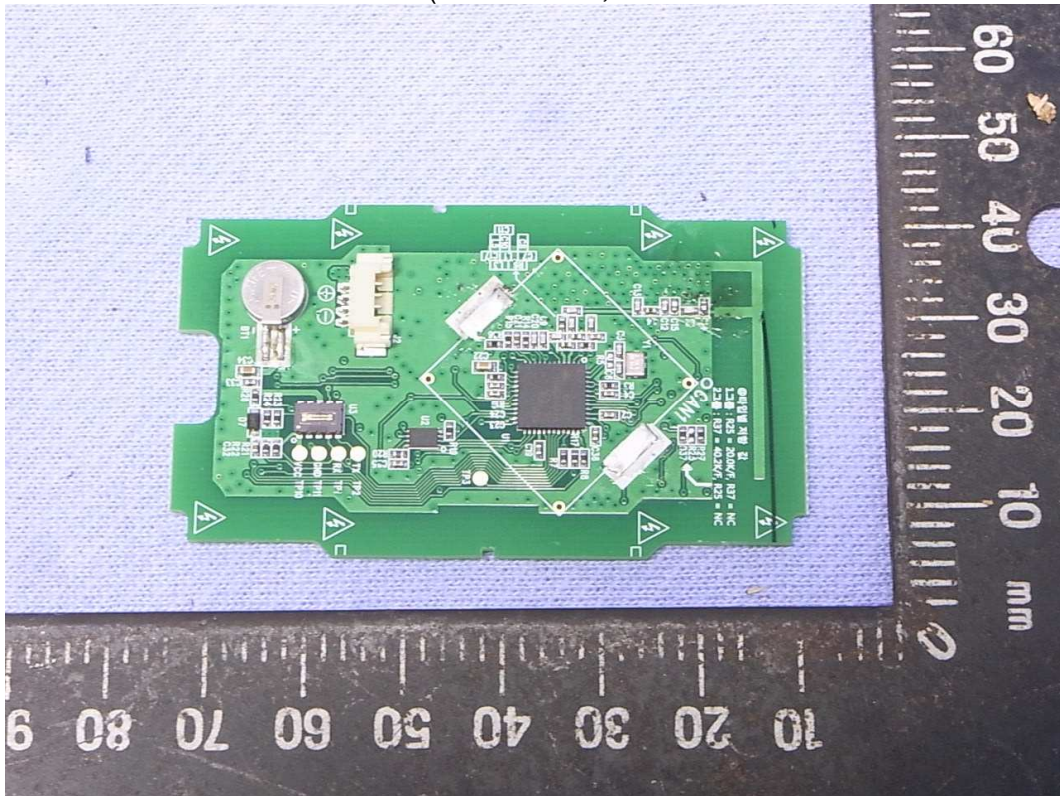
Figure 7 Internal View (Main Board, Front View/Removed Shielded Cover)
