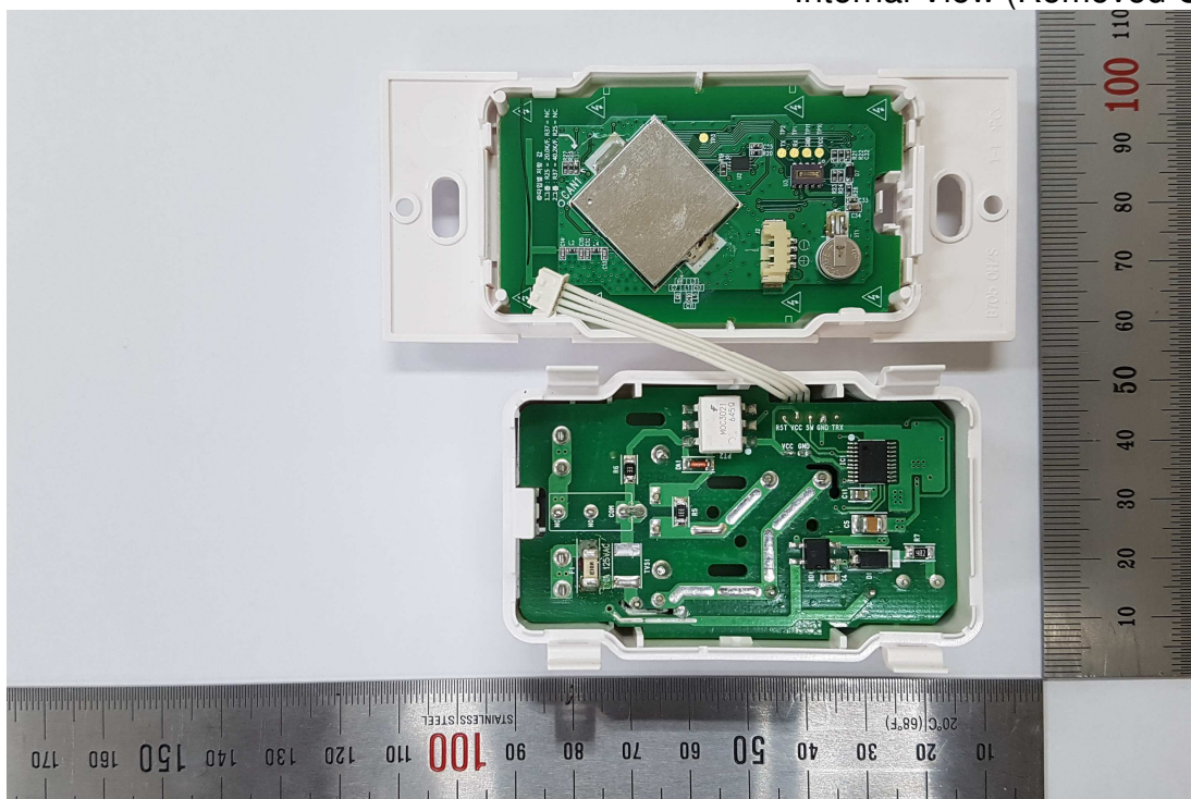
Figure 12 Internal View (Removed Cover)
