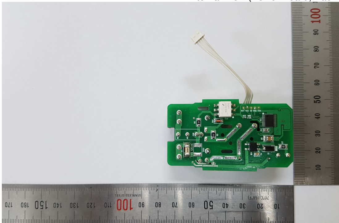
Figure 10 Internal View (Power Board, Back View)
