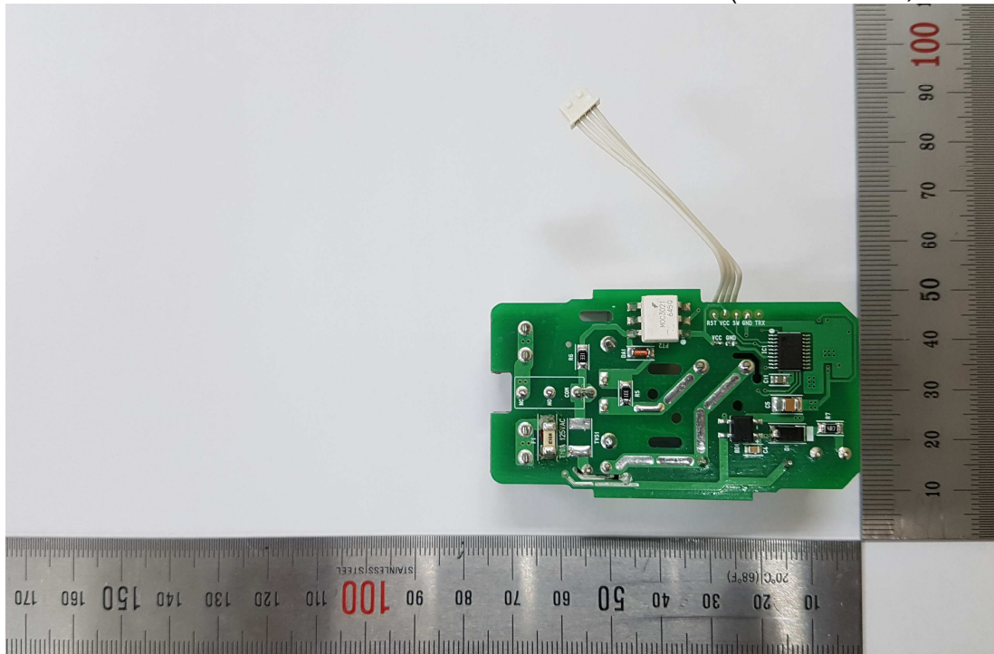
Figure 17 Internal View (Power Board, Back View)
