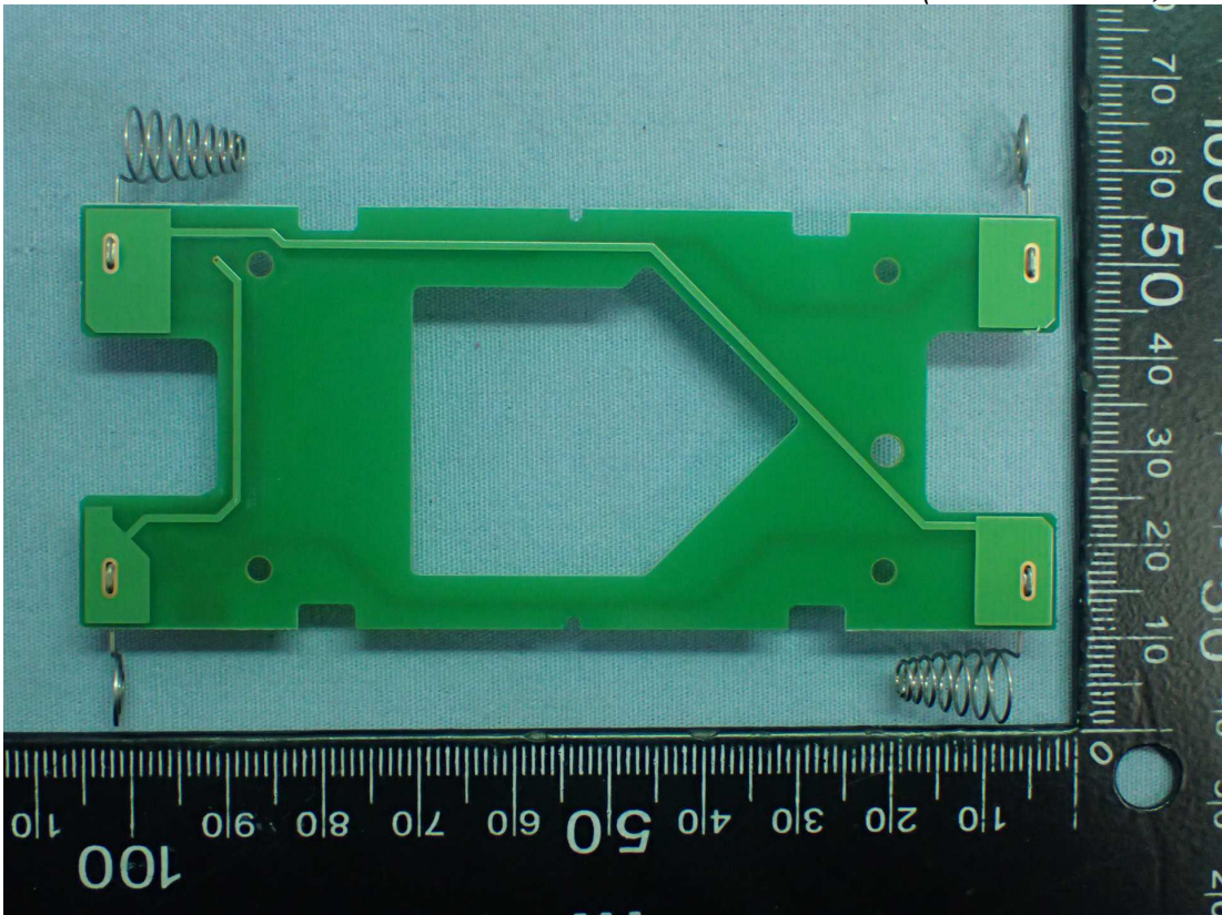
Figure 8 Internal View (Control Board, Back View)
