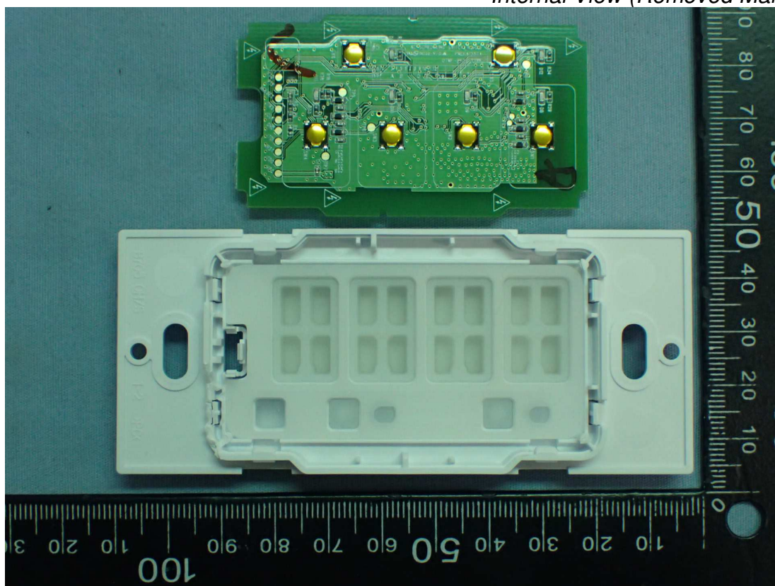
Figure 9 Internal View (Removed Main Board)
