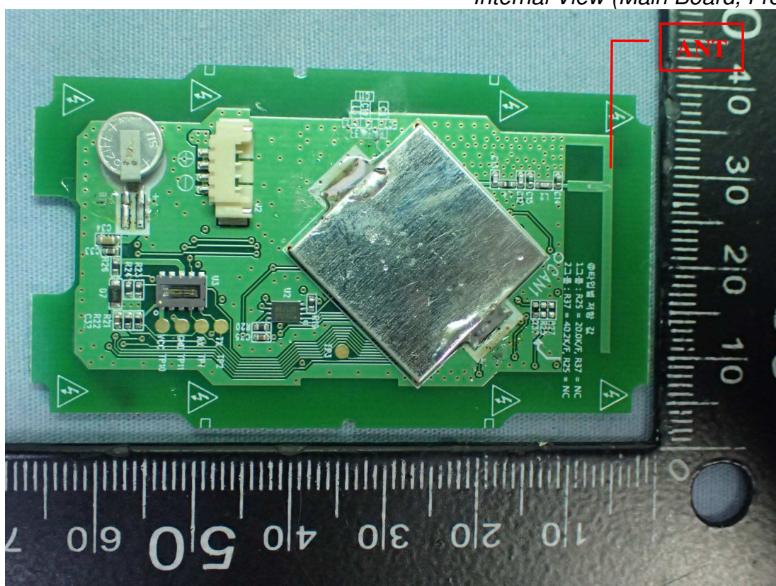
Figure 10 Internal View (Main Board, Front View)
