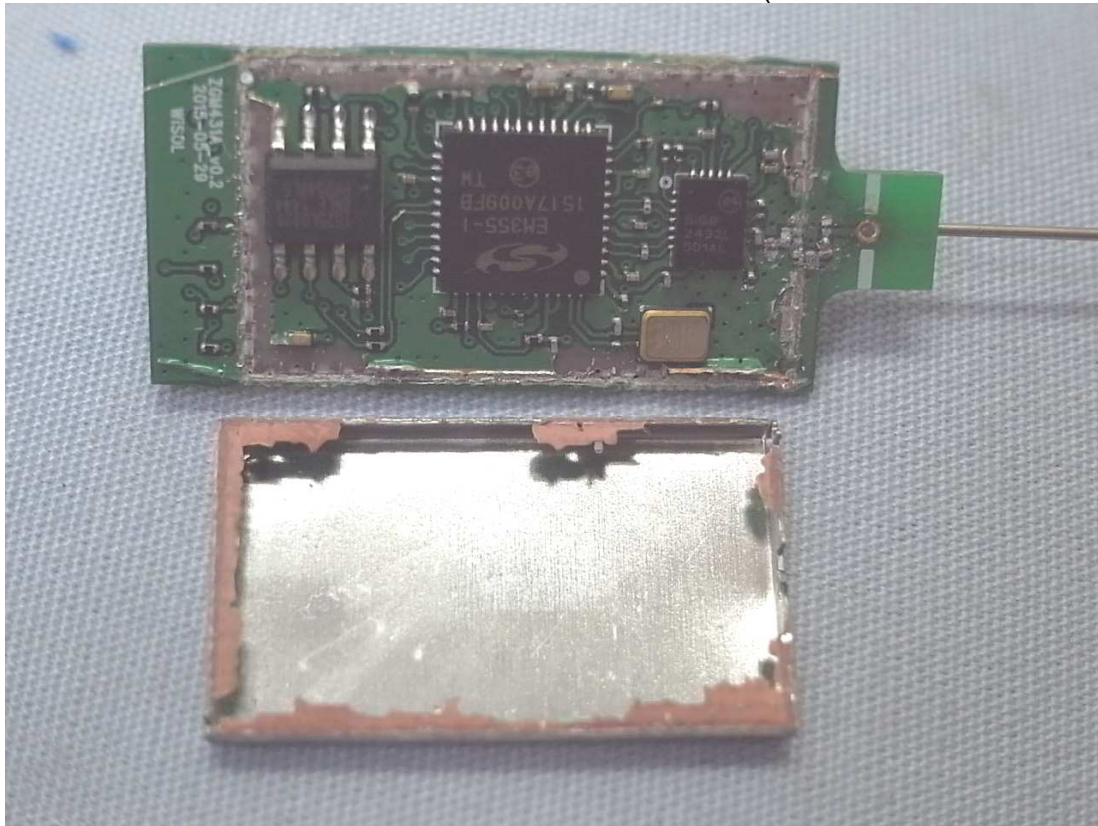
Figure 3 Internal View (Removed Shielded Cover)
