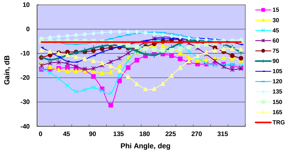
Theta-Polarization Gain
