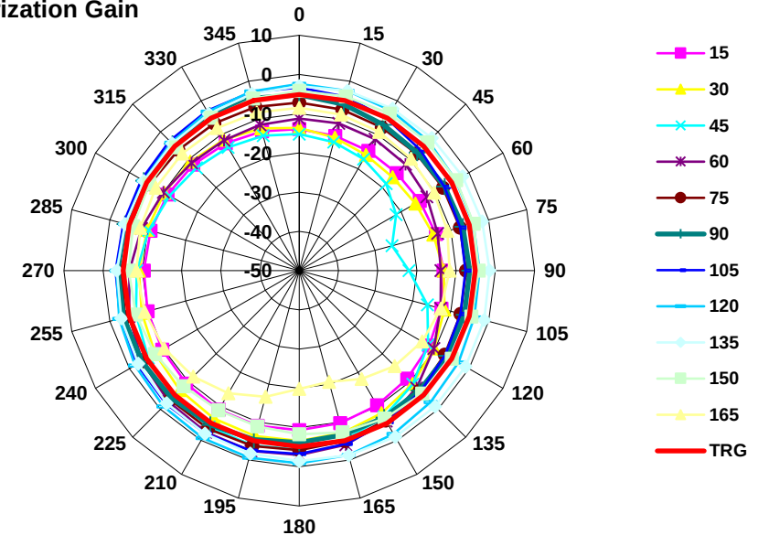
Theta-Polarization + Phi-Polarization Gain
