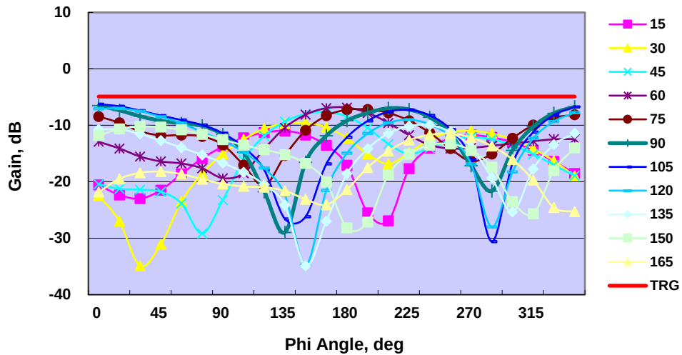
Phi-Polarization Gain
