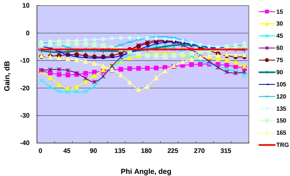
Theta-Polarization + Phi-Polarization Gain
