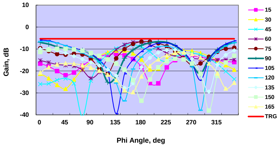
Phi-Polarization Gain
