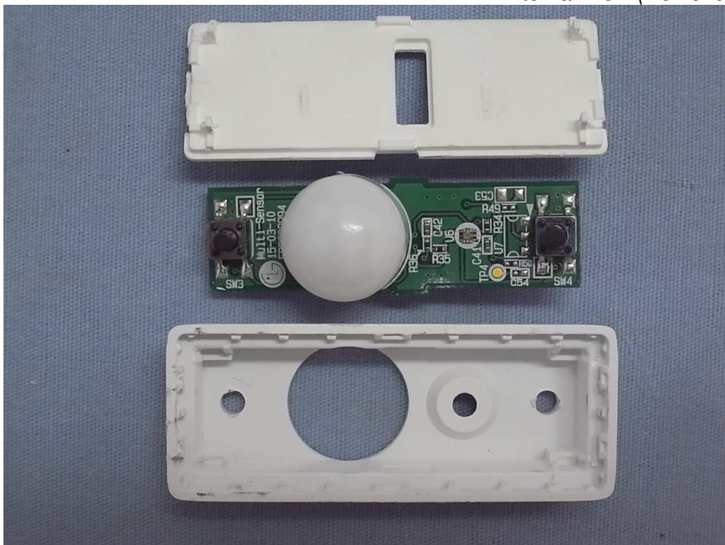
Sensor Figure 9 Internal View (Removed Covers)
