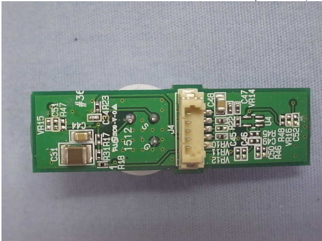
Figure 11 Internal View (Main Board, Back View)
