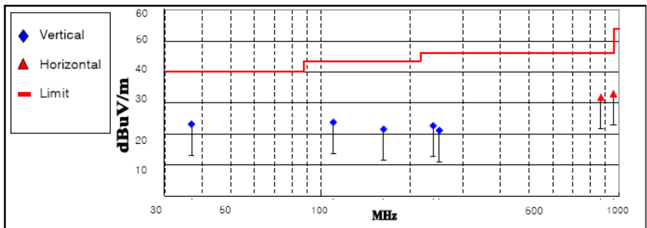
&lt; Fig 5. Radiated Emission result _DVD play mode &gt;
