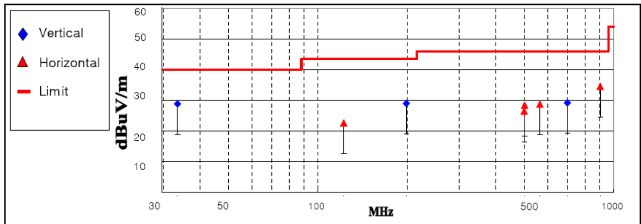
< Fig 4. Radiated emission result _ PC mode >
